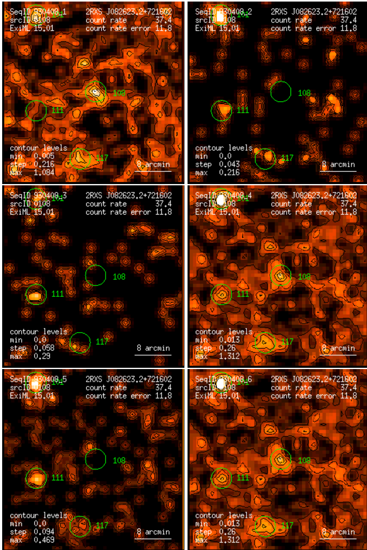
Figure 108: RASS 930408: detection 0108: band rate images, Gaussian filter: (1) PSPC channels 11 – 41, (2) 52 – 90, (3) 91 – 201, (4) 11 – 235, (5) 52 – 201, (6) 11 – 201. Broad band rates in counts/ks. Band rate contour levels in counts/ks/arcmin 2 .
