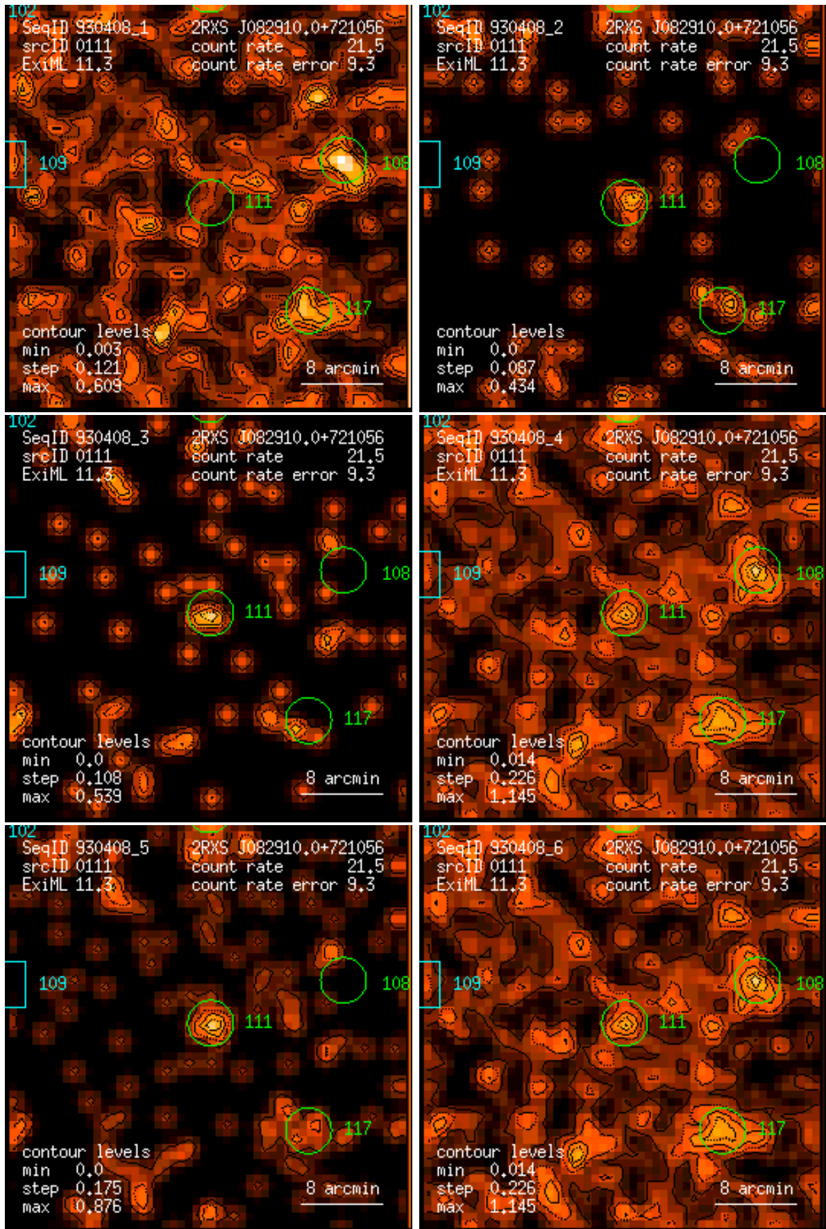
Figure 111: RASS 930408: detection 0111: band rate images, Gaussian filter: (1) PSPC channels 11 – 41, (2) 52 – 90, (3) 91 – 201, (4) 11 – 235, (5) 52 – 201, (6) 11 – 201. Broad band rates in counts/ks. Band rate contour levels in counts/ks/arcmin 2 .
