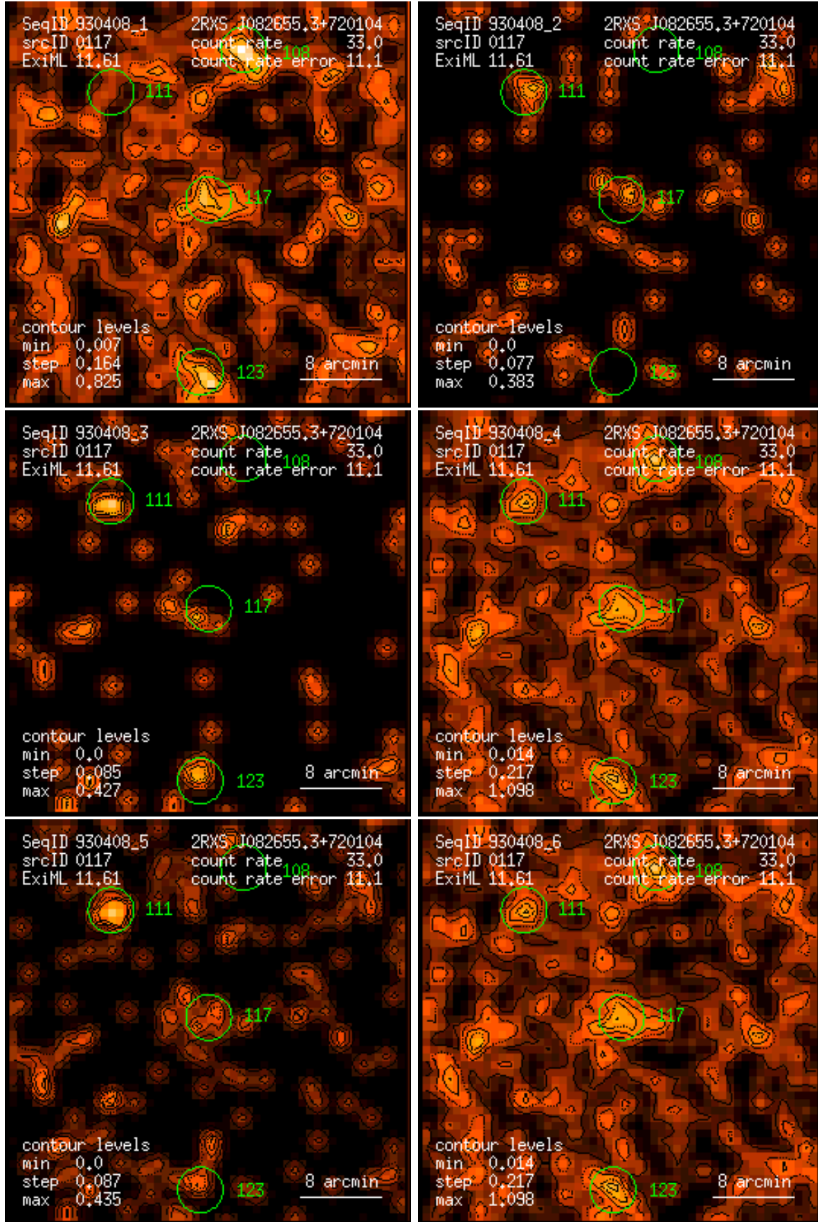
Figure 117: RASS 930408: detection 0117: band rate images, Gaussian filter: (1) PSPC channels 11 – 41, (2) 52 – 90, (3) 91 – 201, (4) 11 – 235, (5) 52 – 201, (6) 11 – 201. Broad band rates in counts/ks. Band rate contour levels in counts/ks/arcmin 2 .
