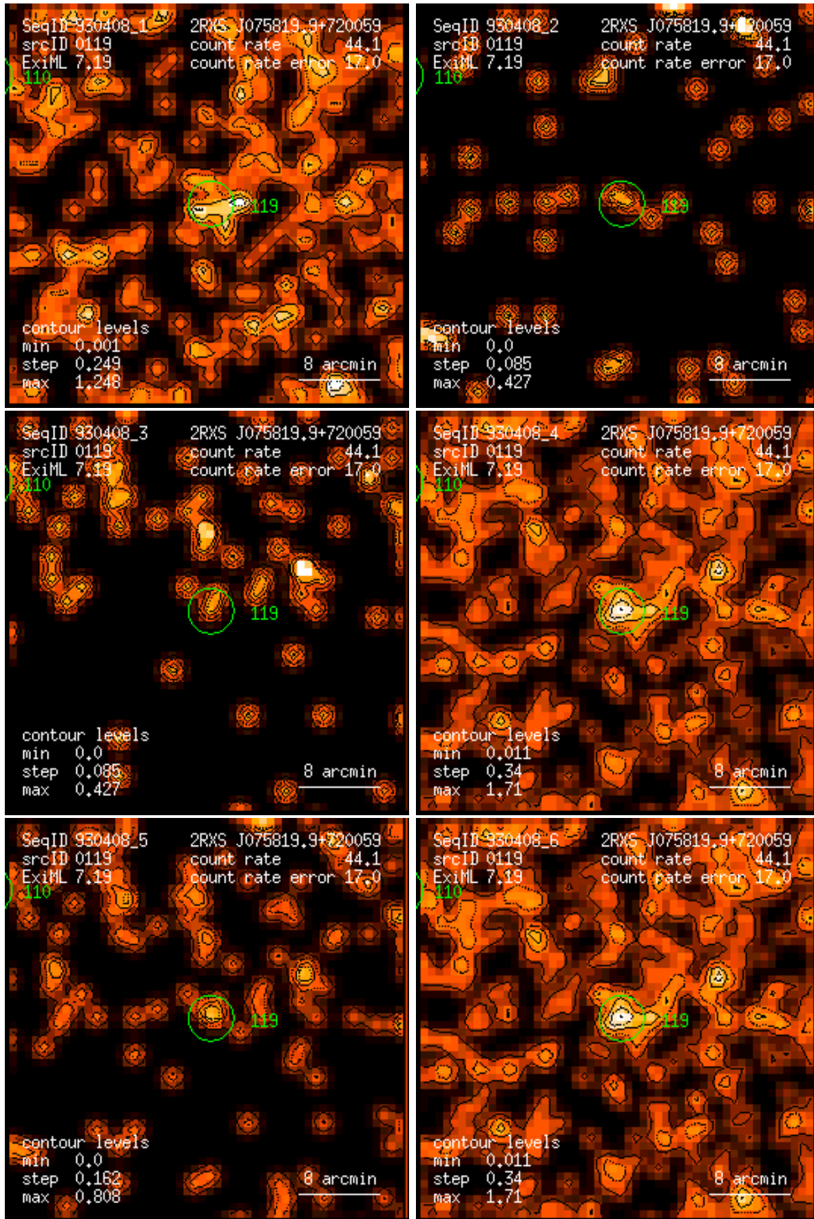
Figure 119: RASS 930408: detection 0119: band rate images, Gaussian filter: (1) PSPC channels 11 – 41, (2) 52 – 90, (3) 91 – 201, (4) 11 – 235, (5) 52 – 201, (6) 11 – 201. Broad band rates in counts/ks. Band rate contour levels in counts/ks/arcmin 2 .
