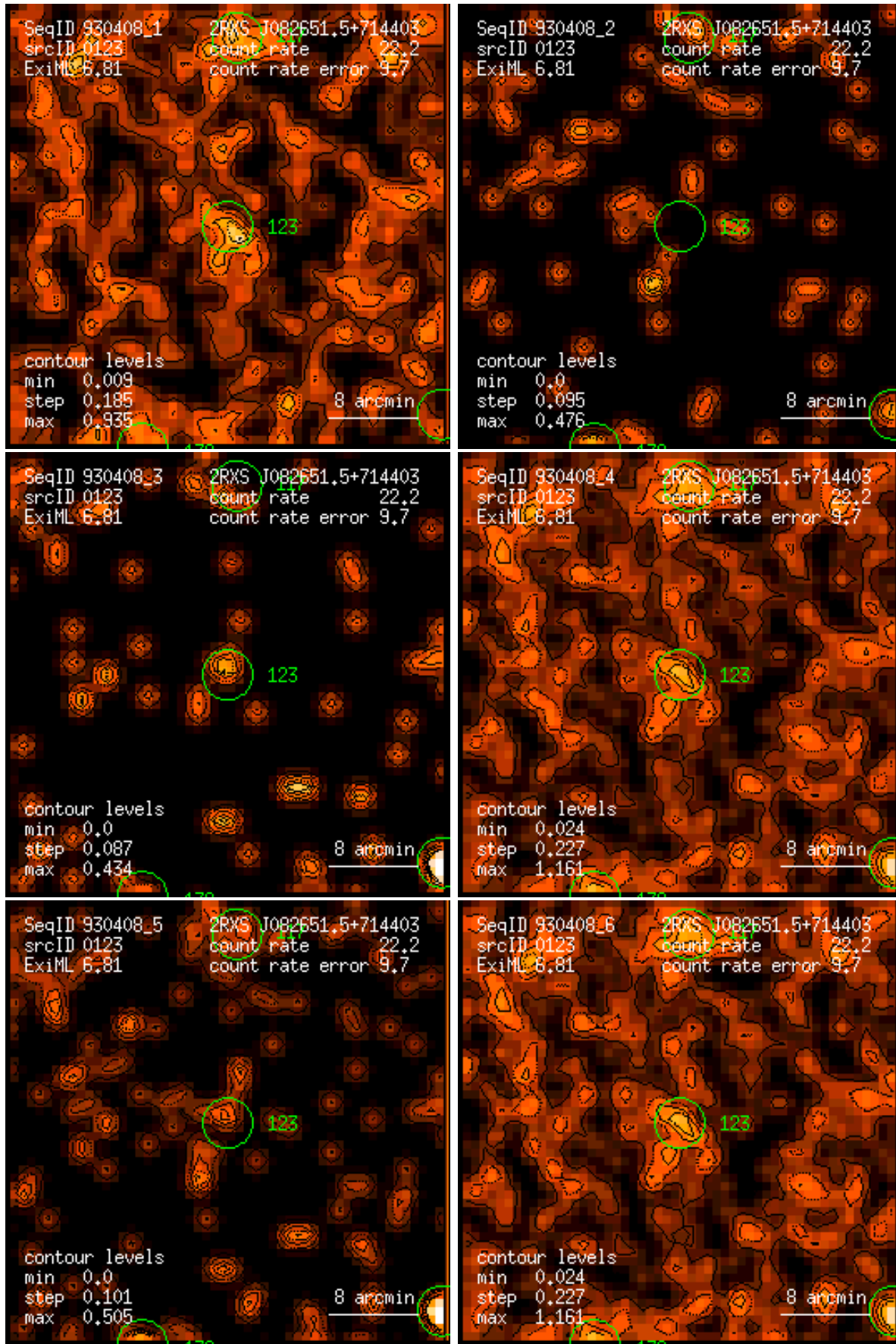
Figure 123: RASS 930408: detection 0123: band rate images, Gaussian filter: (1) PSPC channels 11 – 41, (2) 52 – 90, (3) 91 – 201, (4) 11 – 235, (5) 52 – 201, (6) 11 – 201. Broad band rates in counts/ks. Band rate contour levels in counts/ks/arcmin 2 .
