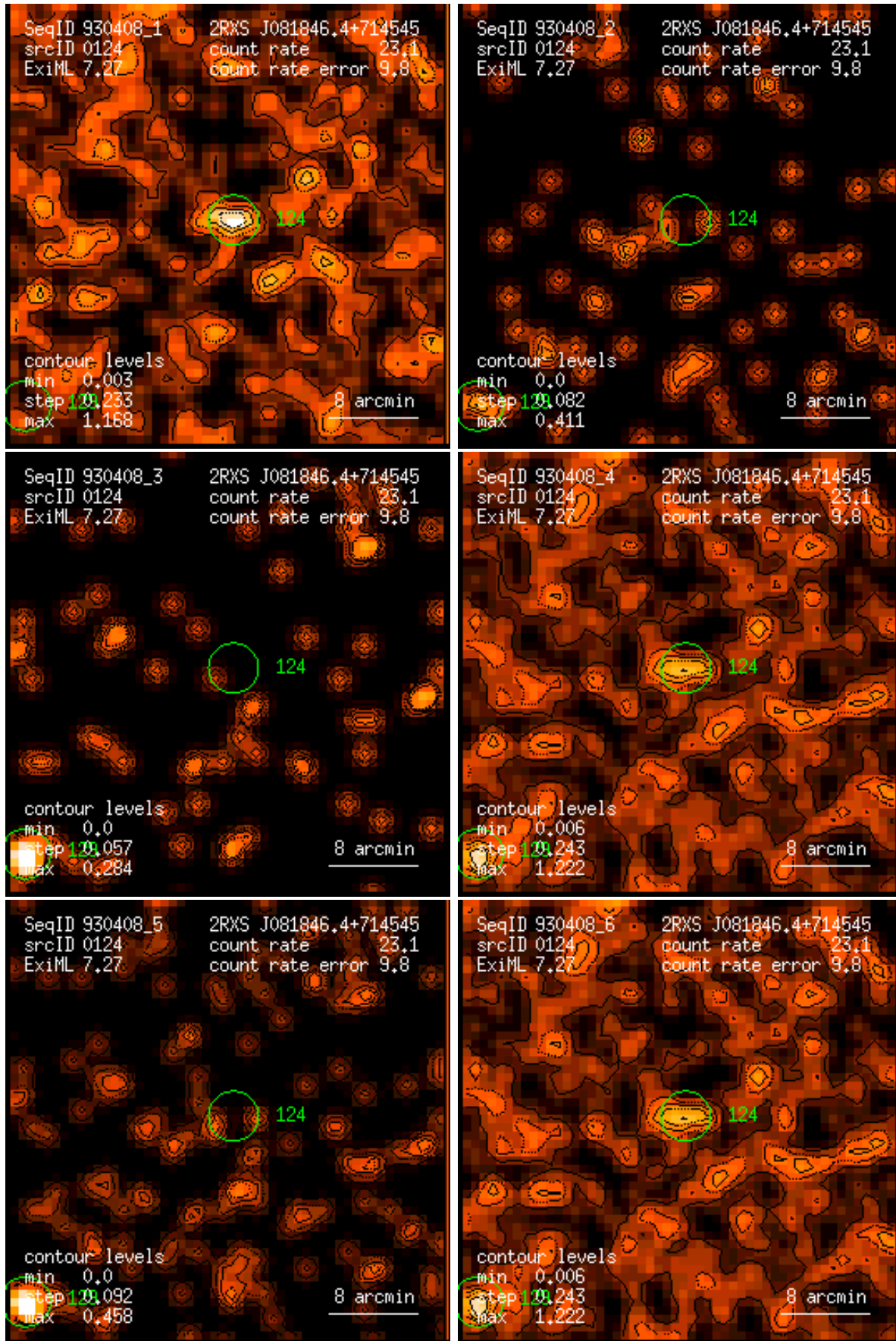
Figure 124: RASS 930408: detection 0124: band rate images, Gaussian filter: (1) PSPC channels 11 – 41, (2) 52 – 90, (3) 91 – 201, (4) 11 – 235, (5) 52 – 201, (6) 11 – 201. Broad band rates in counts/ks. Band rate contour levels in counts/ks/arcmin 2 .
