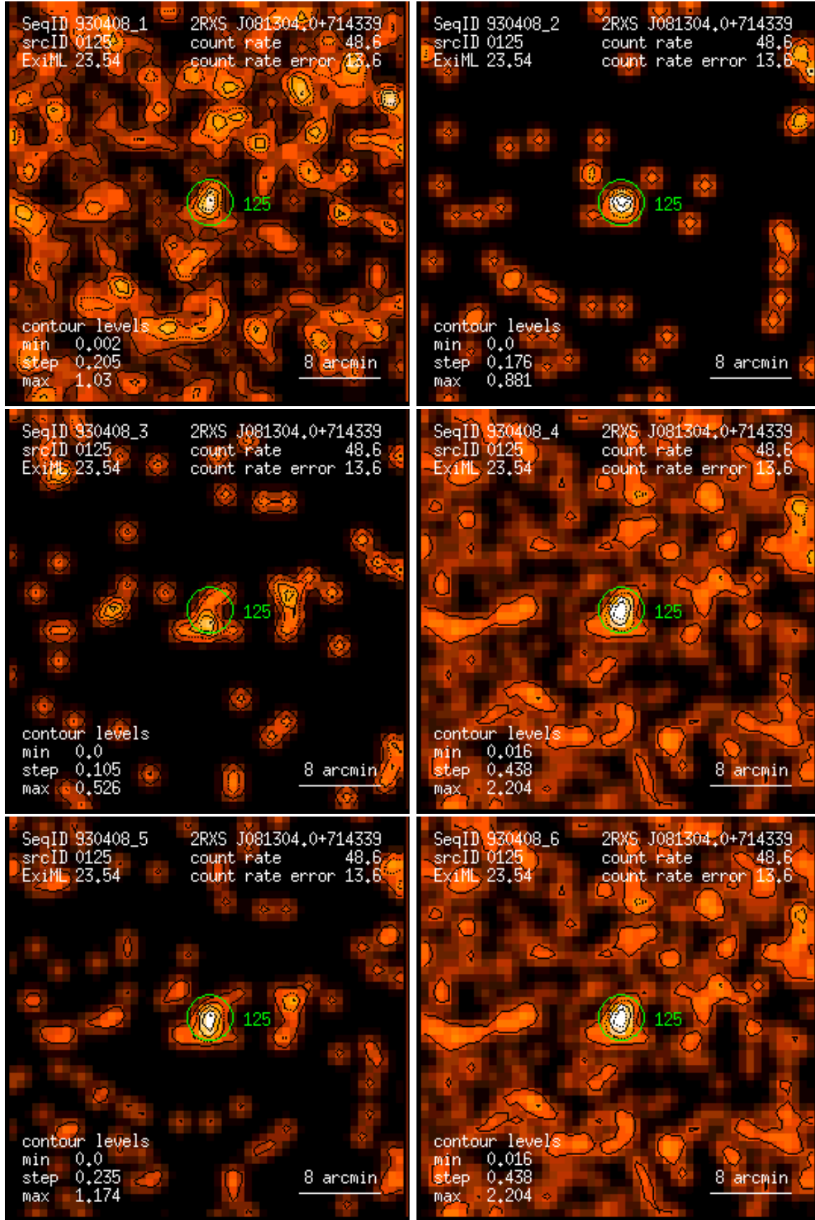
Figure 125: RASS 930408: detection 0125: band rate images, Gaussian filter: (1) PSPC channels 11 – 41, (2) 52 – 90, (3) 91 – 201, (4) 11 – 235, (5) 52 – 201, (6) 11 – 201. Broad band rates in counts/ks. Band rate contour levels in counts/ks/arcmin 2 .
