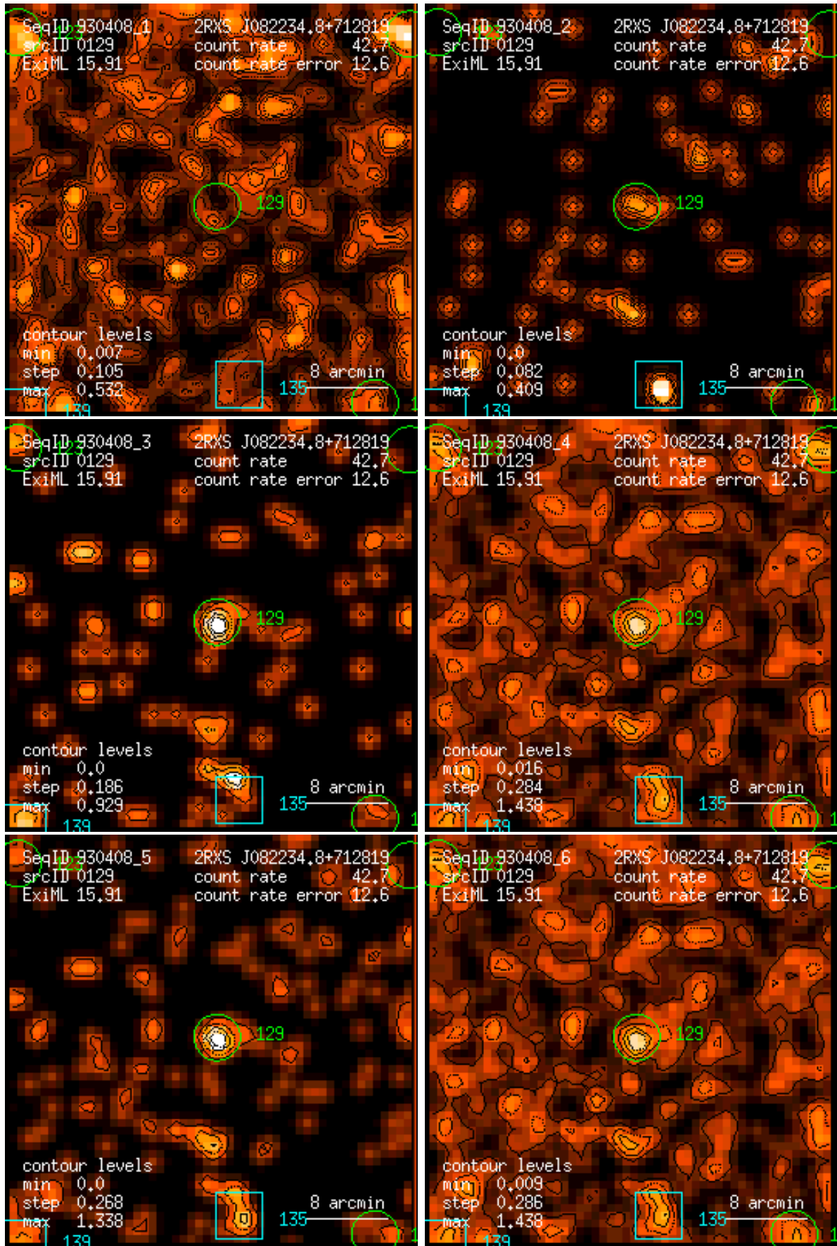
Figure 129: RASS 930408: detection 0129: band rate images, Gaussian filter: (1) PSPC channels 11 – 41, (2) 52 – 90, (3) 91 – 201, (4) 11 – 235, (5) 52 – 201, (6) 11 – 201. Broad band rates in counts/ks. Band rate contour levels in counts/ks/arcmin 2 .
