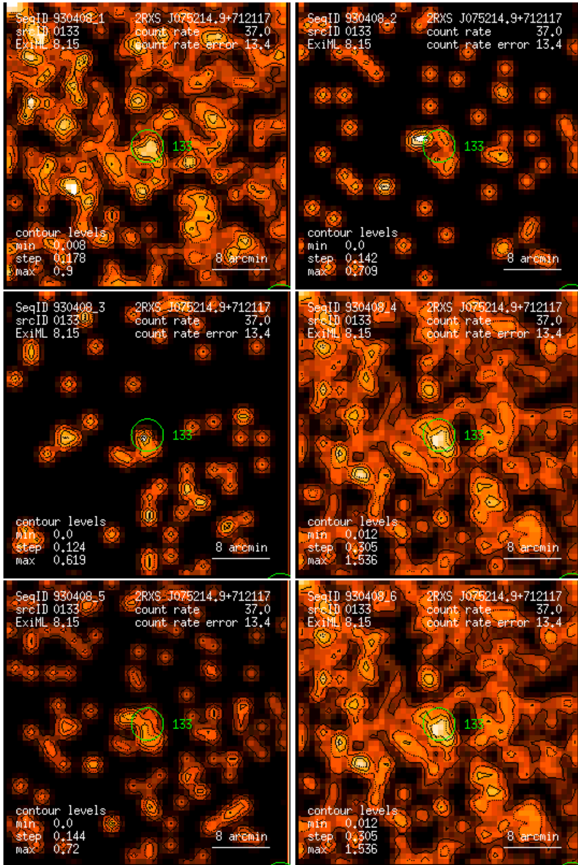
Figure 133: RASS 930408: detection 0133: band rate images, Gaussian filter: (1) PSPC channels 11 – 41, (2) 52 – 90, (3) 91 – 201, (4) 11 – 235, (5) 52 – 201, (6) 11 – 201. Broad band rates in counts/ks. Band rate contour levels in counts/ks/arcmin 2 .
