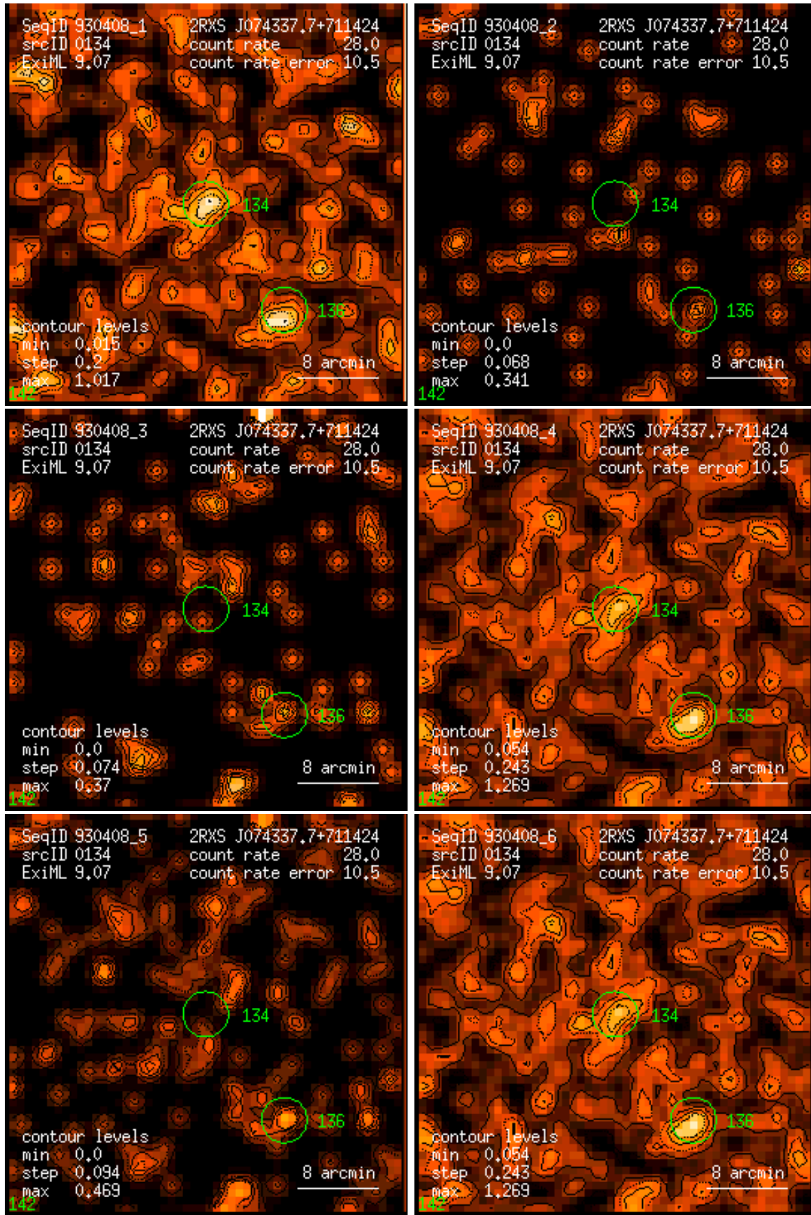
Figure 134: RASS 930408: detection 0134: band rate images, Gaussian filter: (1) PSPC channels 11 – 41, (2) 52 – 90, (3) 91 – 201, (4) 11 – 235, (5) 52 – 201, (6) 11 – 201. Broad band rates in counts/ks. Band rate contour levels in counts/ks/arcmin 2 .
