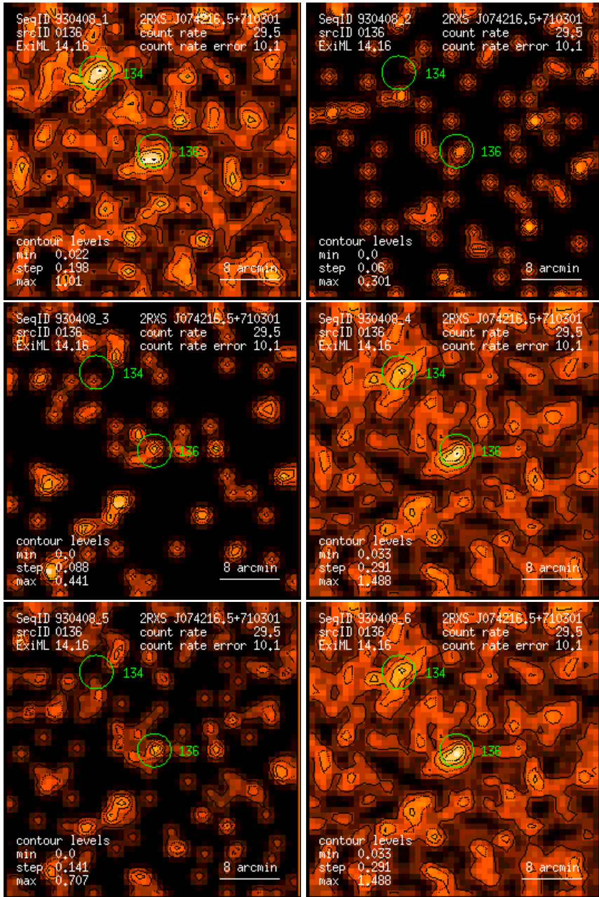
Figure 136: RASS 930408: detection 0136: band rate images, Gaussian filter: (1) PSPC channels 11 – 41, (2) 52 – 90, (3) 91 – 201, (4) 11 – 235, (5) 52 – 201, (6) 11 – 201. Broad band rates in counts/ks. Band rate contour levels in counts/ks/arcmin 2 .
