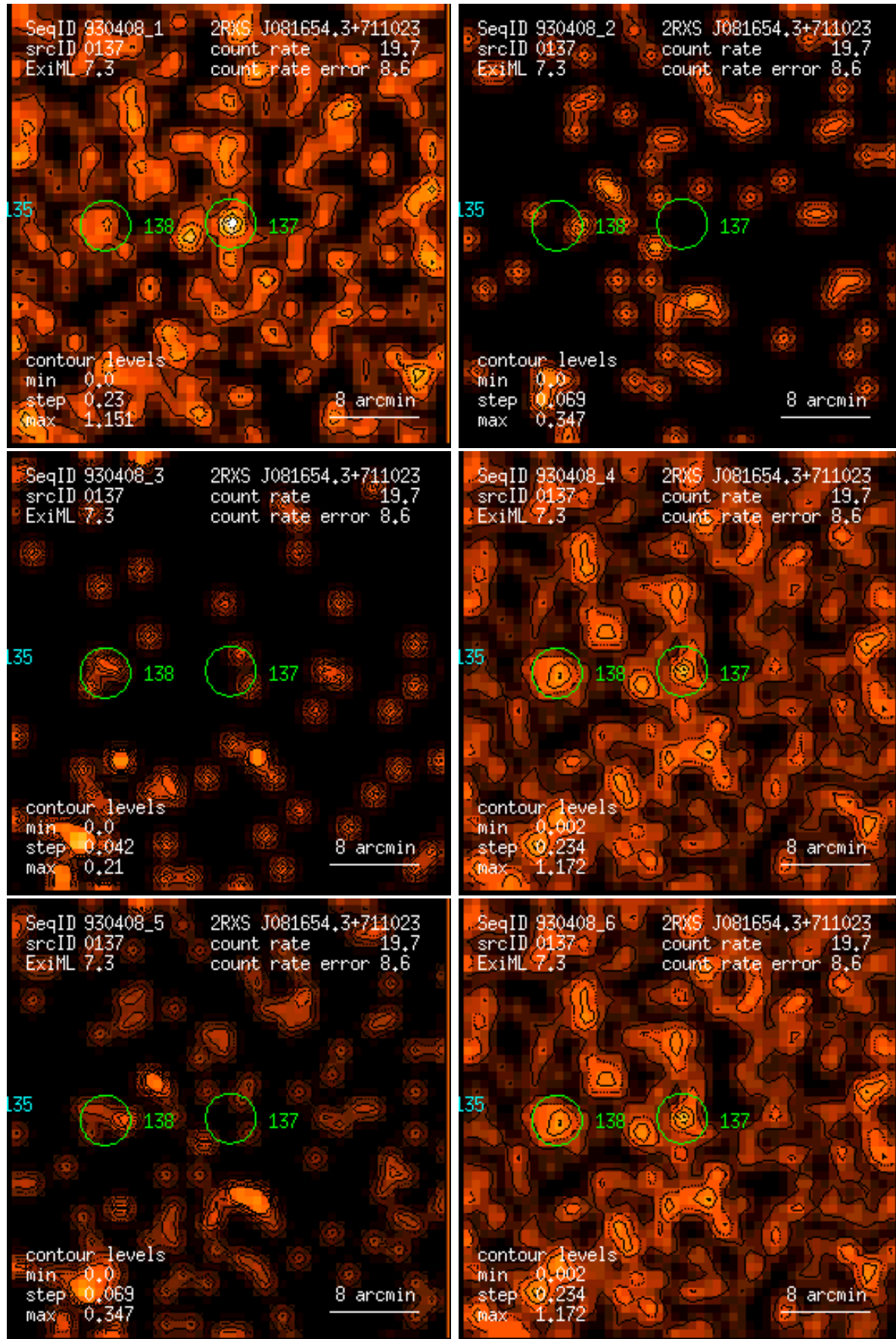
Figure 137: RASS 930408: detection 0137: band rate images, Gaussian filter: (1) PSPC channels 11 – 41, (2) 52 – 90, (3) 91 – 201, (4) 11 – 235, (5) 52 – 201, (6) 11 – 201. Broad band rates in counts/ks. Band rate contour levels in counts/ks/arcmin 2 .
