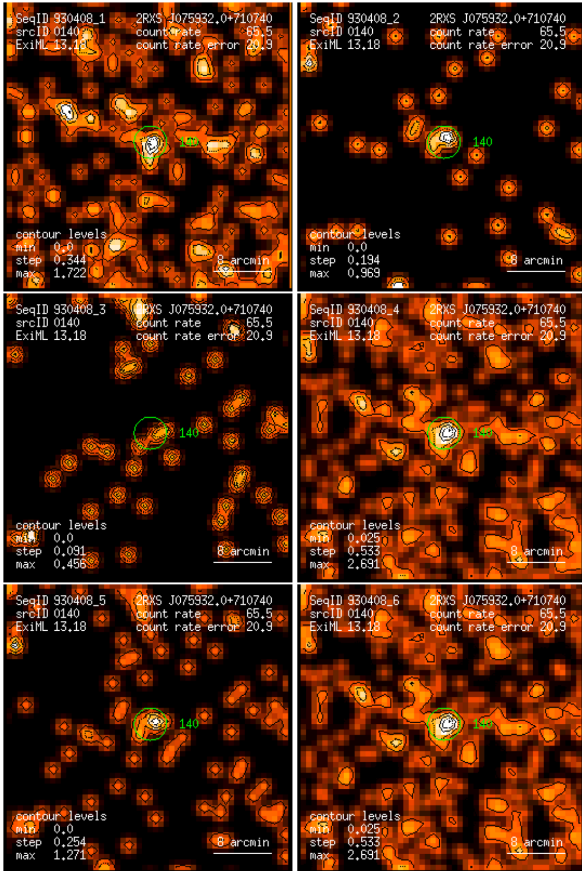
Figure 140: RASS 930408: detection 0140: band rate images, Gaussian filter: (1) PSPC channels 11 – 41, (2) 52 – 90, (3) 91 – 201, (4) 11 – 235, (5) 52 – 201, (6) 11 – 201. Broad band rates in counts/ks. Band rate contour levels in counts/ks/arcmin 2 .
