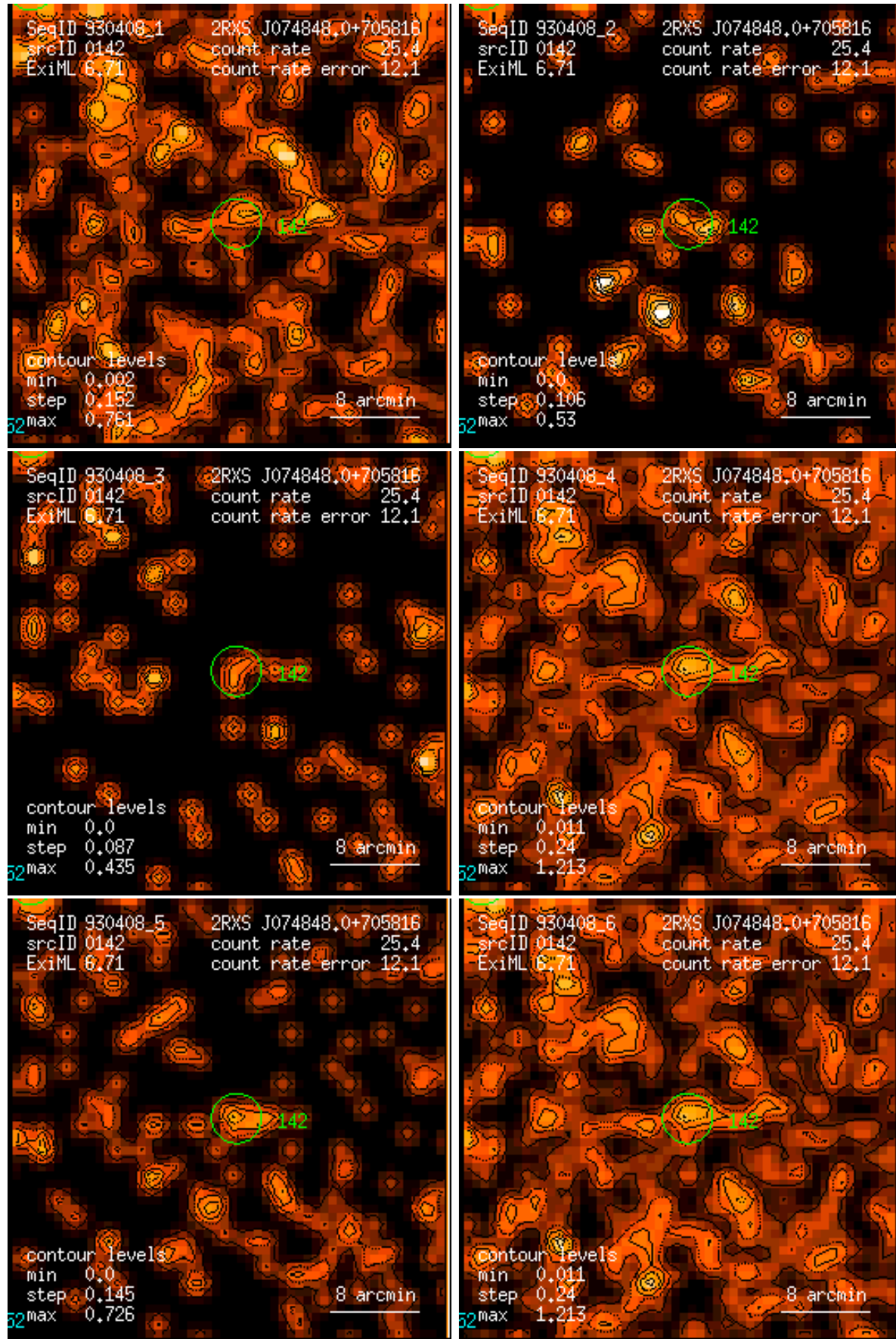
Figure 142: RASS 930408: detection 0142: band rate images, Gaussian filter: (1) PSPC channels 11 – 41, (2) 52 – 90, (3) 91 – 201, (4) 11 – 235, (5) 52 – 201, (6) 11 – 201. Broad band rates in counts/ks. Band rate contour levels in counts/ks/arcmin 2 .
