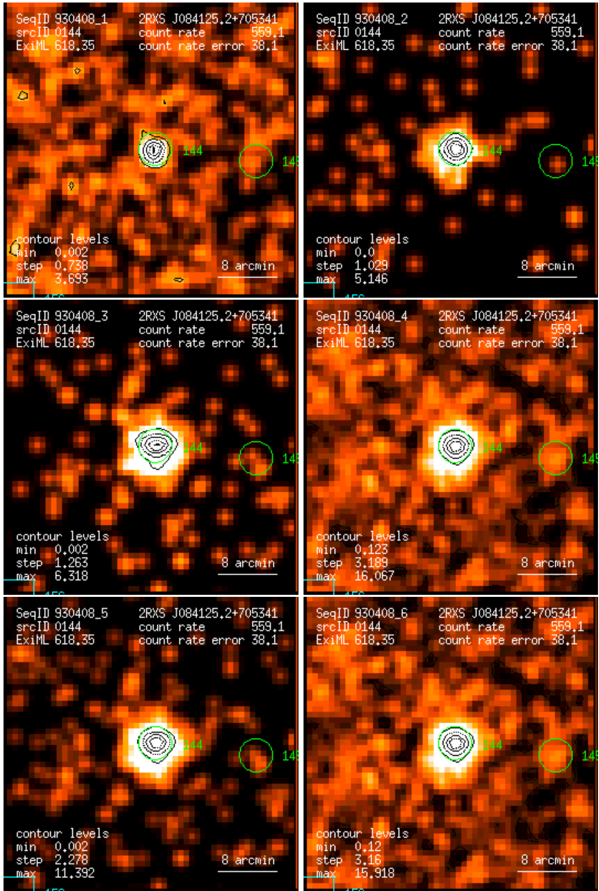
Figure 144: RASS 930408: detection 0144: band rate images, Gaussian filter: (1) PSPC channels 11 – 41, (2) 52 – 90, (3) 91 – 201, (4) 11 – 235, (5) 52 – 201, (6) 11 – 201. Broad band rates in counts/ks. Band rate contour levels in counts/ks/arcmin 2 .
