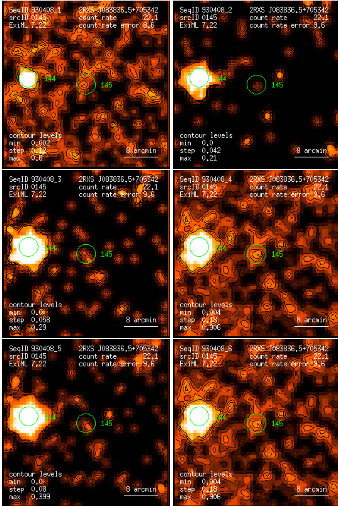
Figure 145: RASS 930408: detection 0145: band rate images, Gaussian filter: (1) PSPC channels 11 – 41, (2) 52 – 90, (3) 91 – 201, (4) 11 – 235, (5) 52 – 201, (6) 11 – 201. Broad band rates in counts/ks. Band rate contour levels in counts/ks/arcmin 2 .
