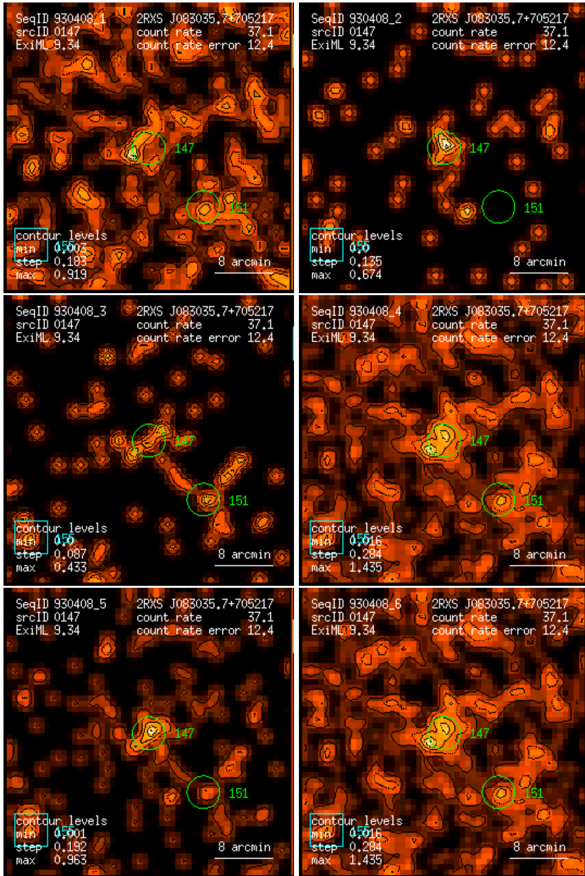
Figure 147: RASS 930408: detection 0147: band rate images, Gaussian filter: (1) PSPC channels 11 – 41, (2) 52 – 90, (3) 91 – 201, (4) 11 – 235, (5) 52 – 201, (6) 11 – 201. Broad band rates in counts/ks. Band rate contour levels in counts/ks/arcmin 2 .
