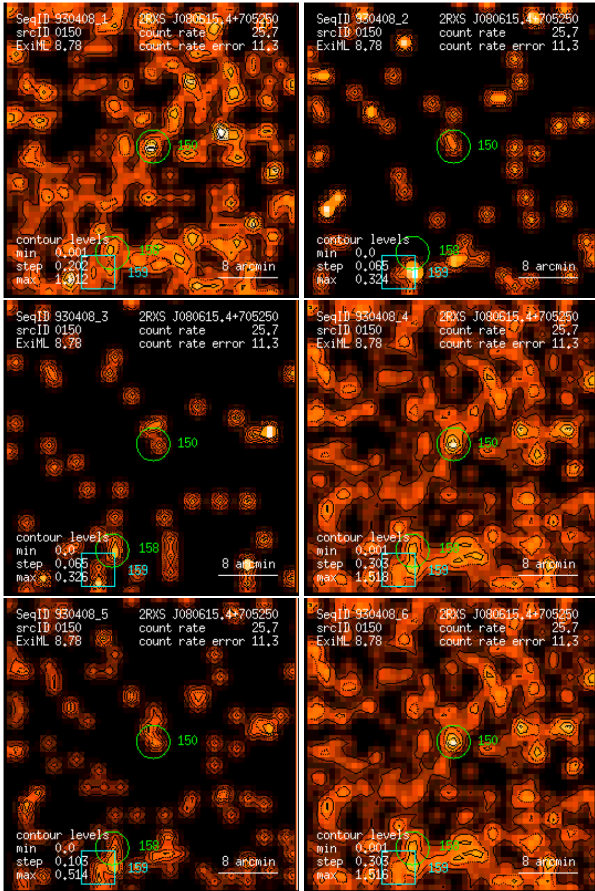
Figure 150: RASS 930408: detection 0150: band rate images, Gaussian filter: (1) PSPC channels 11 – 41, (2) 52 – 90, (3) 91 – 201, (4) 11 – 235, (5) 52 – 201, (6) 11 – 201. Broad band rates in counts/ks. Band rate contour levels in counts/ks/arcmin 2 .
