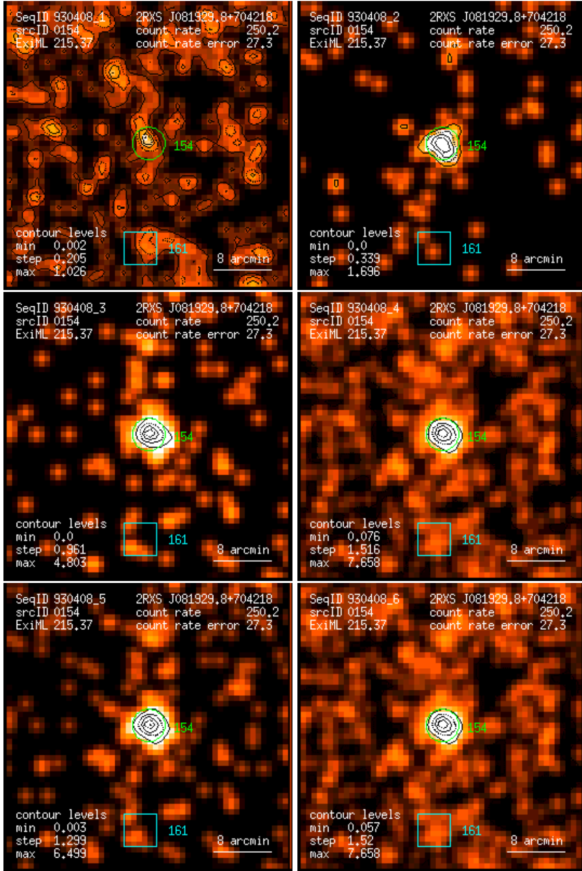
Figure 154: RASS 930408: detection 0154: band rate images, Gaussian filter: (1) PSPC channels 11 – 41, (2) 52 – 90, (3) 91 – 201, (4) 11 – 235, (5) 52 – 201, (6) 11 – 201. Broad band rates in counts/ks. Band rate contour levels in counts/ks/arcmin 2 .
