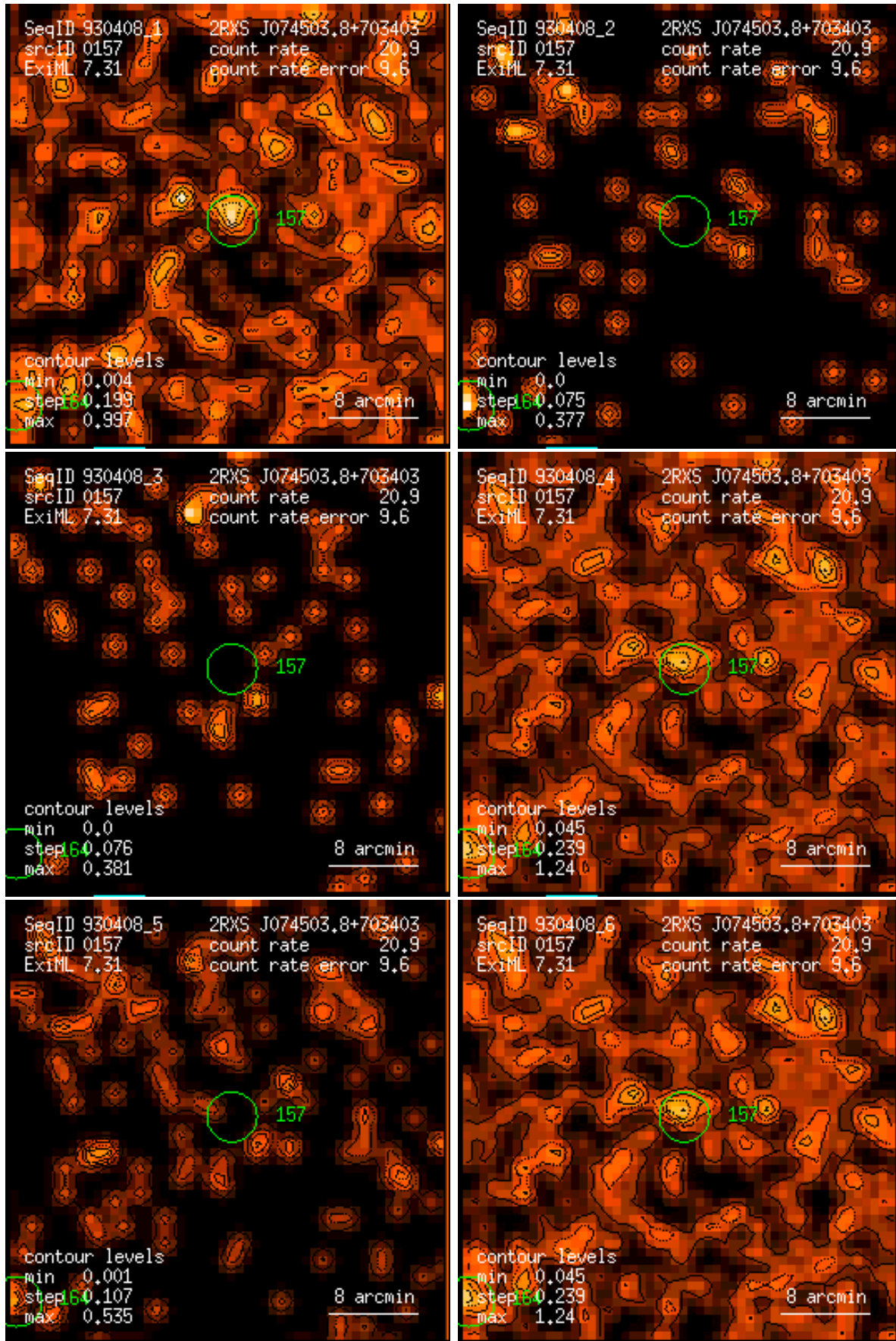
Figure 157: RASS 930408: detection 0157: band rate images, Gaussian filter: (1) PSPC channels 11 – 41, (2) 52 – 90, (3) 91 – 201, (4) 11 – 235, (5) 52 – 201, (6) 11 – 201. Broad band rates in counts/ks. Band rate contour levels in counts/ks/arcmin 2 .
