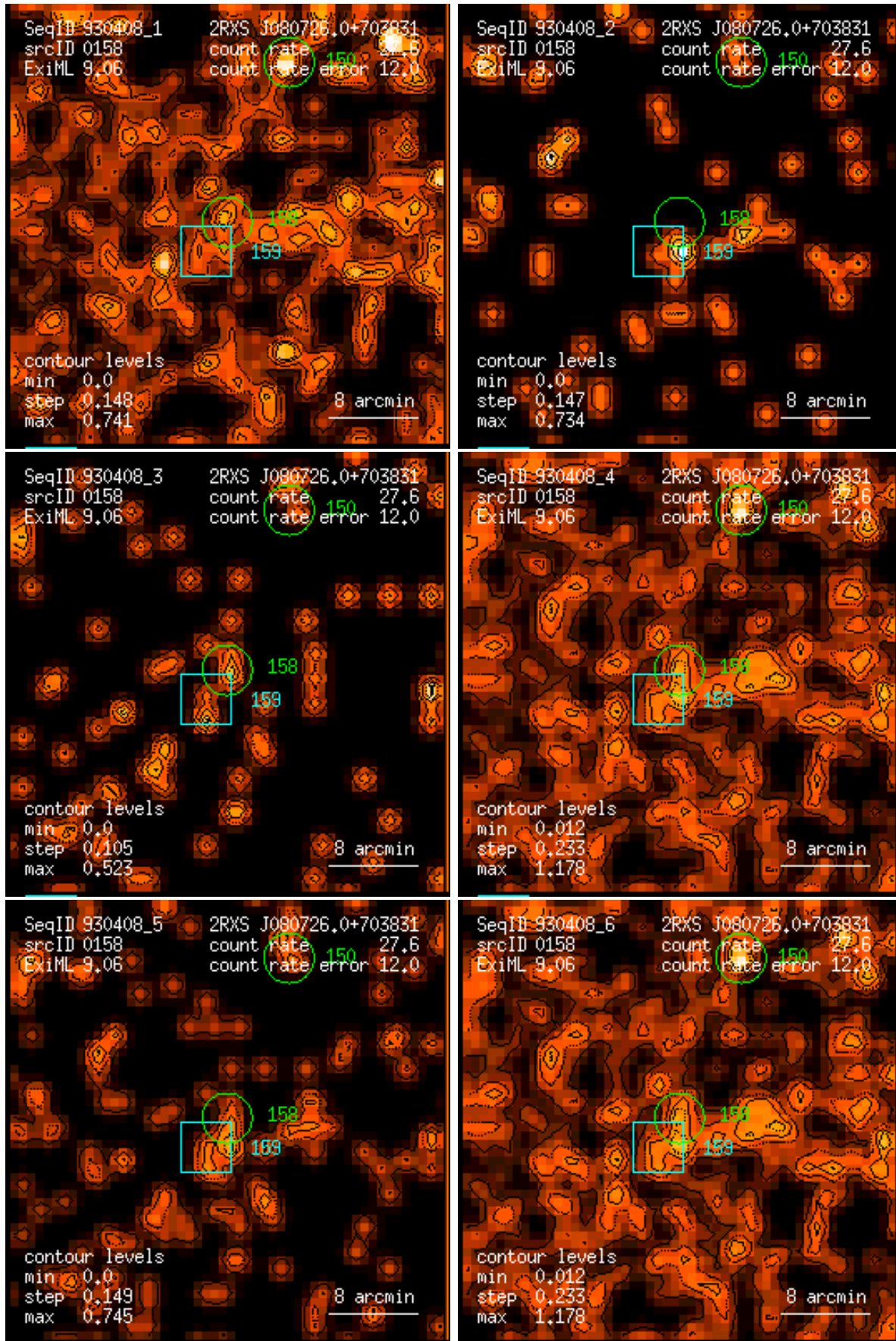
Figure 158: RASS 930408: detection 0158: band rate images, Gaussian filter: (1) PSPC channels 11 – 41, (2) 52 – 90, (3) 91 – 201, (4) 11 – 235, (5) 52 – 201, (6) 11 – 201. Broad band rates in counts/ks. Band rate contour levels in counts/ks/arcmin 2 .
