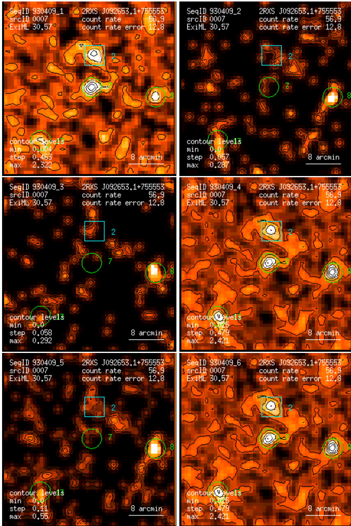
Figure 7: RASS 930409: detection 0007: band rate images, Gaussian filter: (1) PSPC channels 11 – 41, (2) 52 – 90, (3) 91 – 201, (4) 11 – 235, (5) 52 – 201, (6) 11 – 201. Broad band rates in counts/ks. Band rate contour levels in counts/ks/arcmin 2 .
