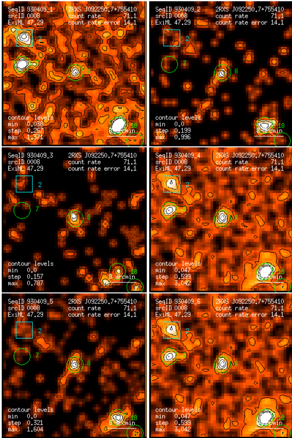
Figure 8: RASS 930409: detection 0008: band rate images, Gaussian filter: (1) PSPC channels 11 – 41, (2) 52 – 90, (3) 91 – 201, (4) 11 – 235, (5) 52 – 201, (6) 11 – 201. Broad band rates in counts/ks. Band rate contour levels in counts/ks/arcmin 2 .
