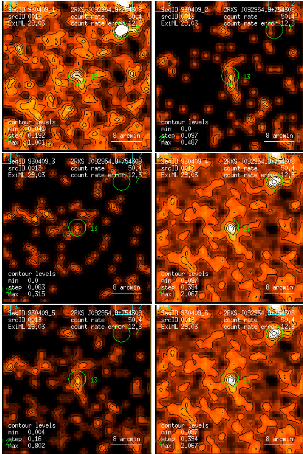
Figure 13: RASS 930409: detection 0013: band rate images, Gaussian filter: (1) PSPC channels 11 – 41, (2) 52 – 90, (3) 91 – 201, (4) 11 – 235, (5) 52 – 201, (6) 11 – 201. Broad band rates in counts/ks. Band rate contour levels in counts/ks/arcmin 2 .
