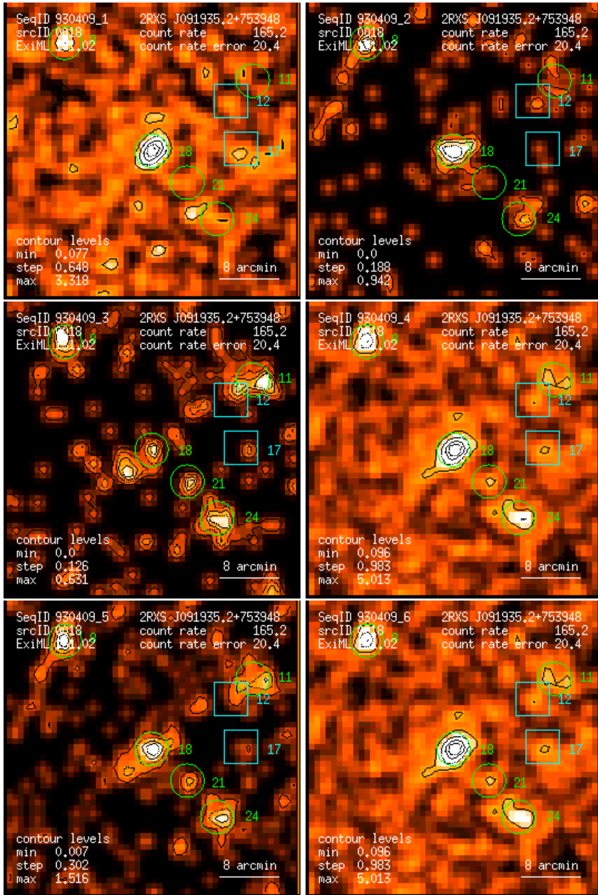
Figure 18: RASS 930409: detection 0018: band rate images, Gaussian filter: (1) PSPC channels 11 – 41, (2) 52 – 90, (3) 91 – 201, (4) 11 – 235, (5) 52 – 201, (6) 11 – 201. Broad band rates in counts/ks. Band rate contour levels in counts/ks/arcmin 2 .
