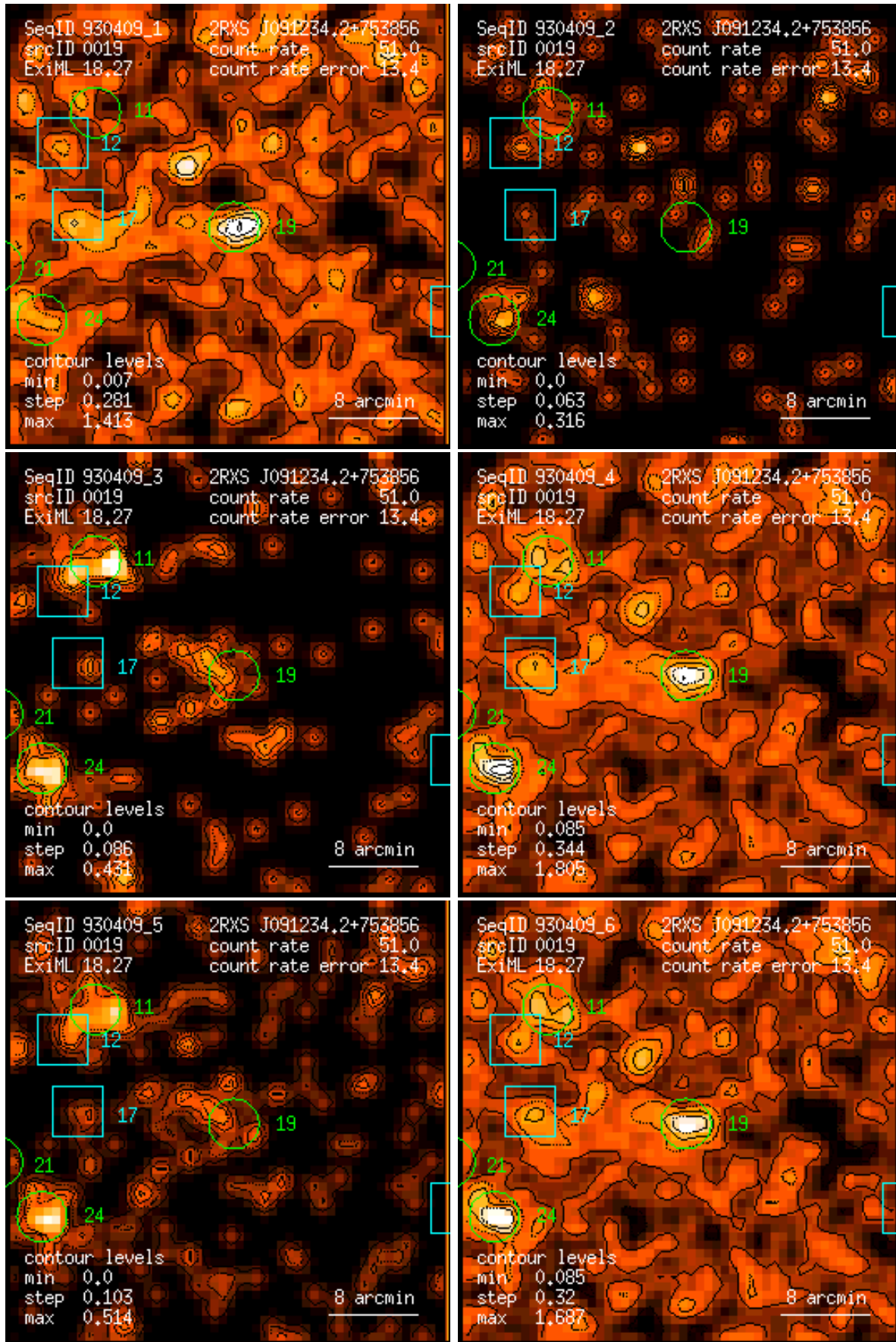
Figure 19: RASS 930409: detection 0019: band rate images, Gaussian filter: (1) PSPC channels 11 – 41, (2) 52 – 90, (3) 91 – 201, (4) 11 – 235, (5) 52 – 201, (6) 11 – 201. Broad band rates in counts/ks. Band rate contour levels in counts/ks/arcmin 2 .
