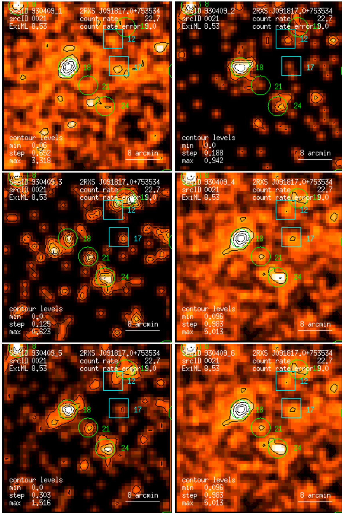
Figure 21: RASS 930409: detection 0021: band rate images, Gaussian filter: (1) PSPC channels 11 – 41, (2) 52 – 90, (3) 91 – 201, (4) 11 – 235, (5) 52 – 201, (6) 11 – 201. Broad band rates in counts/ks. Band rate contour levels in counts/ks/arcmin 2 .
