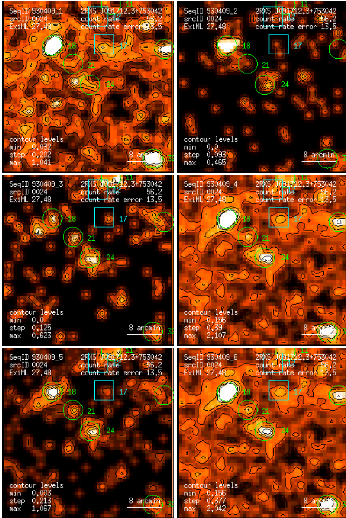
Figure 24: RASS 930409: detection 0024: band rate images, Gaussian filter: (1) PSPC channels 11 – 41, (2) 52 – 90, (3) 91 – 201, (4) 11 – 235, (5) 52 – 201, (6) 11 – 201. Broad band rates in counts/ks. Band rate contour levels in counts/ks/arcmin 2 .
