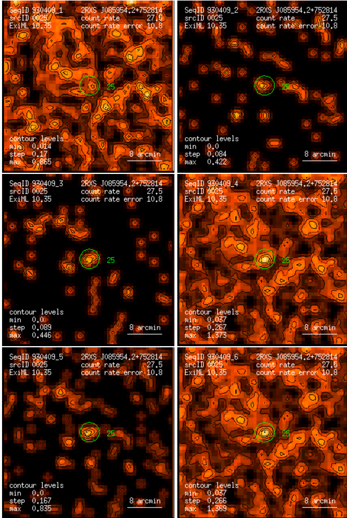
Figure 25: RASS 930409: detection 0025: band rate images, Gaussian filter: (1) PSPC channels 11 – 41, (2) 52 – 90, (3) 91 – 201, (4) 11 – 235, (5) 52 – 201, (6) 11 – 201. Broad band rates in counts/ks. Band rate contour levels in counts/ks/arcmin 2 .
