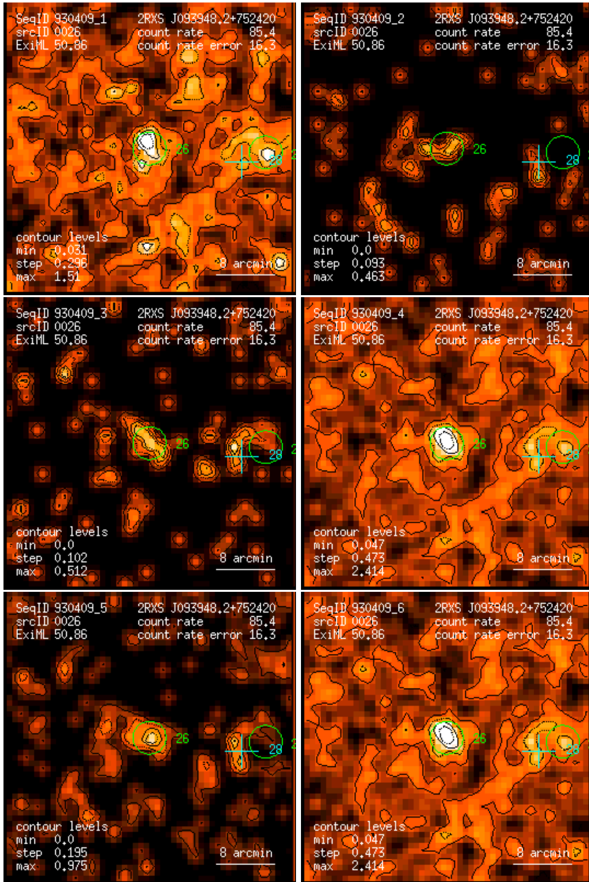
Figure 26: RASS 930409: detection 0026: band rate images, Gaussian filter: (1) PSPC channels 11 – 41, (2) 52 – 90, (3) 91 – 201, (4) 11 – 235, (5) 52 – 201, (6) 11 – 201. Broad band rates in counts/ks. Band rate contour levels in counts/ks/arcmin 2 .
