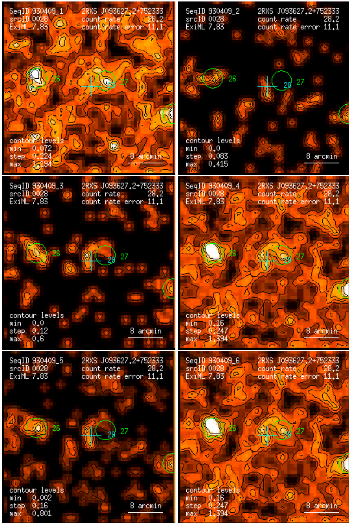
Figure 28: RASS 930409: detection 0028: band rate images, Gaussian filter: (1) PSPC channels 11 – 41, (2) 52 – 90, (3) 91 – 201, (4) 11 – 235, (5) 52 – 201, (6) 11 – 201. Broad band rates in counts/ks. Band rate contour levels in counts/ks/arcmin 2 .
