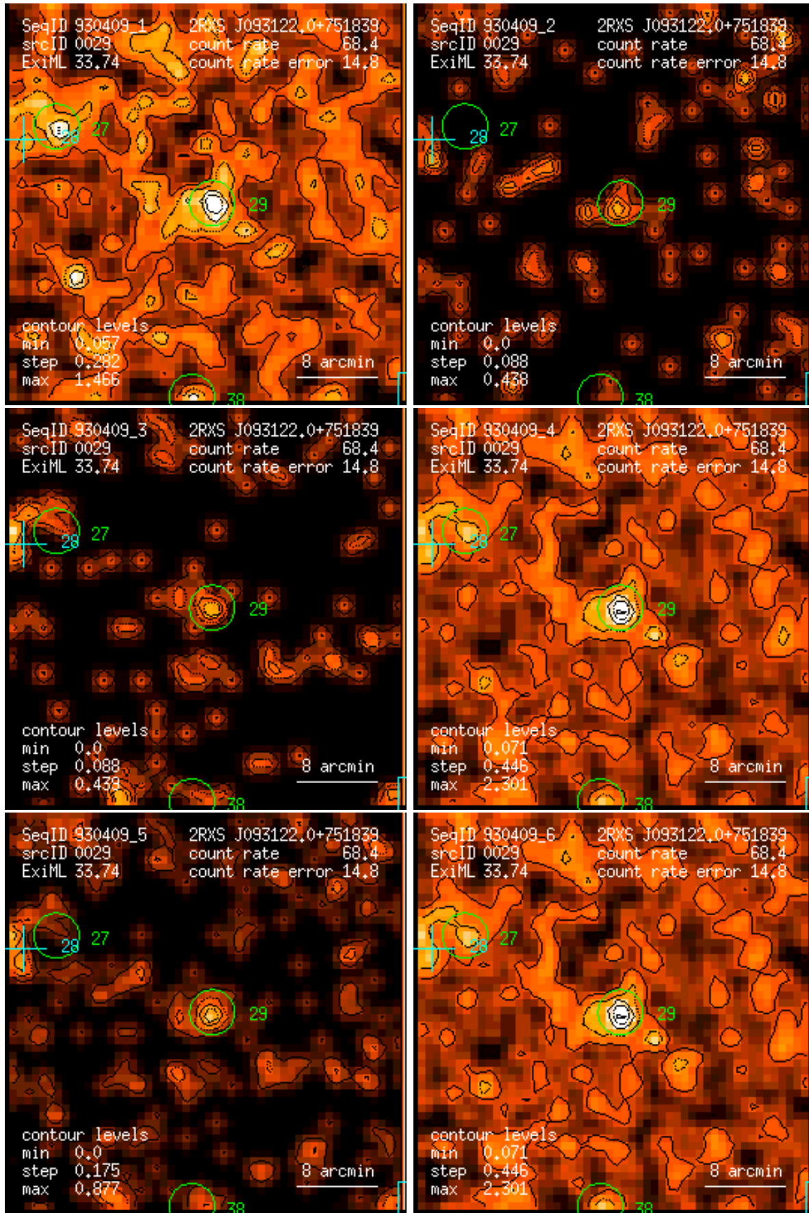
Figure 29: RASS 930409: detection 0029: band rate images, Gaussian filter: (1) PSPC channels 11 – 41, (2) 52 – 90, (3) 91 – 201, (4) 11 – 235, (5) 52 – 201, (6) 11 – 201. Broad band rates in counts/ks. Band rate contour levels in counts/ks/arcmin 2 .
