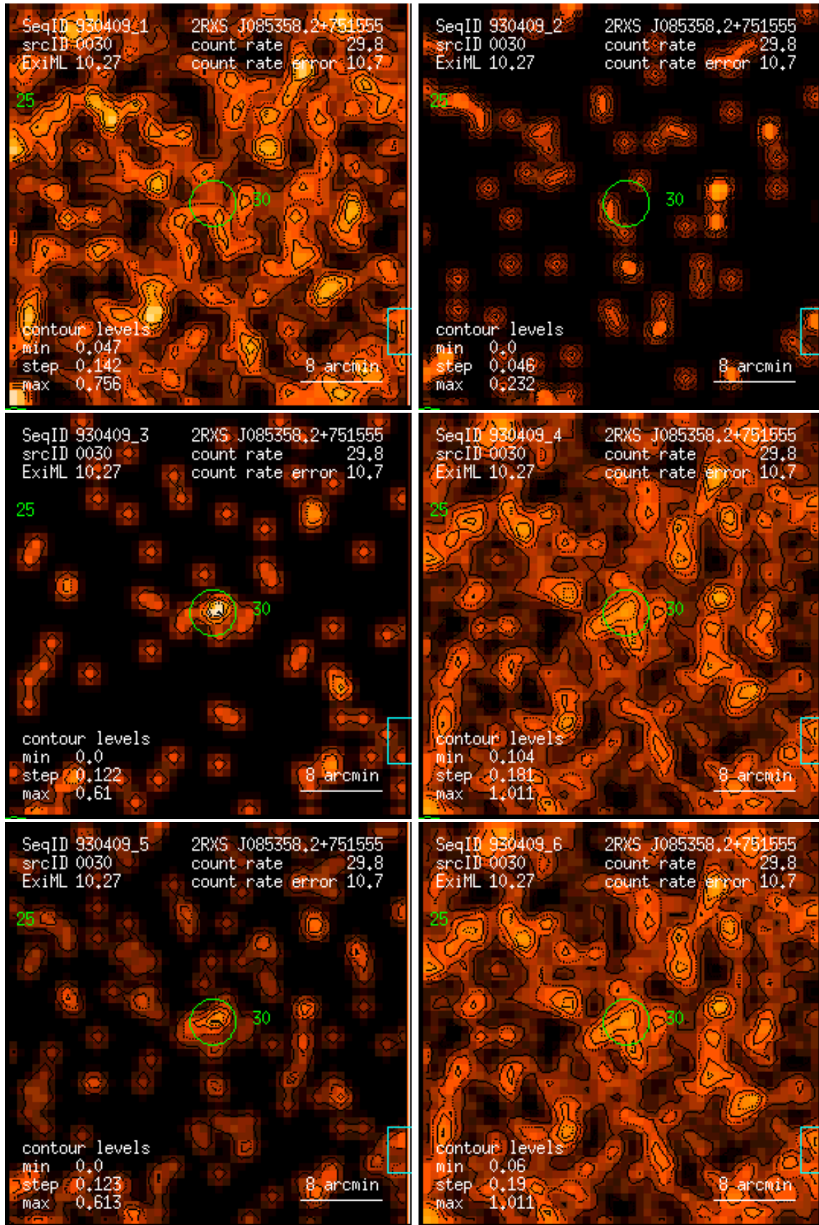
Figure 30: RASS 930409: detection 0030: band rate images, Gaussian filter: (1) PSPC channels 11 – 41, (2) 52 – 90, (3) 91 – 201, (4) 11 – 235, (5) 52 – 201, (6) 11 – 201. Broad band rates in counts/ks. Band rate contour levels in counts/ks/arcmin 2 .
