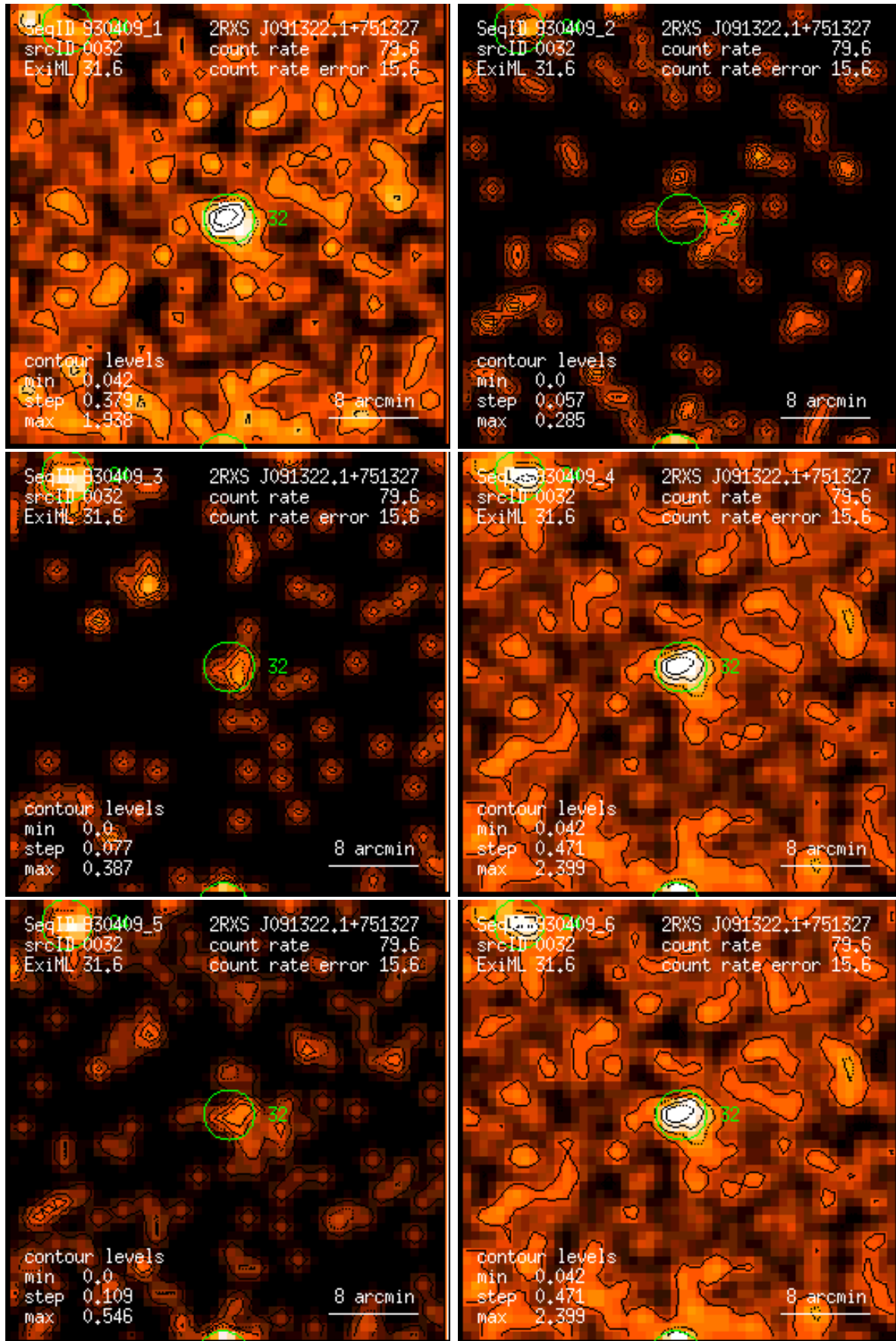
Figure 32: RASS 930409: detection 0032: band rate images, Gaussian filter: (1) PSPC channels 11 – 41, (2) 52 – 90, (3) 91 – 201, (4) 11 – 235, (5) 52 – 201, (6) 11 – 201. Broad band rates in counts/ks. Band rate contour levels in counts/ks/arcmin 2 .
