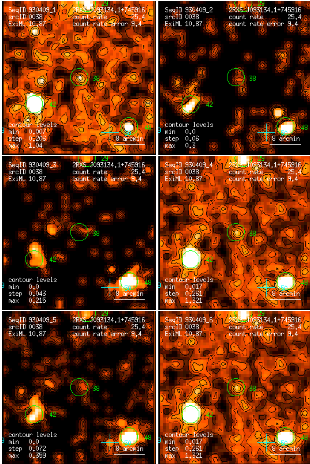
Figure 38: RASS 930409: detection 0038: band rate images, Gaussian filter: (1) PSPC channels 11 – 41, (2) 52 – 90, (3) 91 – 201, (4) 11 – 235, (5) 52 – 201, (6) 11 – 201. Broad band rates in counts/ks. Band rate contour levels in counts/ks/arcmin 2 .
