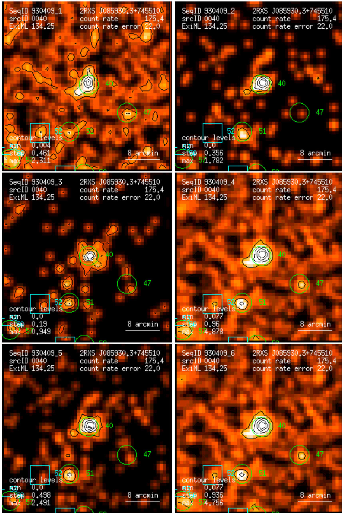
Figure 40: RASS 930409: detection 0040: band rate images, Gaussian filter: (1) PSPC channels 11 – 41, (2) 52 – 90, (3) 91 – 201, (4) 11 – 235, (5) 52 – 201, (6) 11 – 201. Broad band rates in counts/ks. Band rate contour levels in counts/ks/arcmin 2 .
