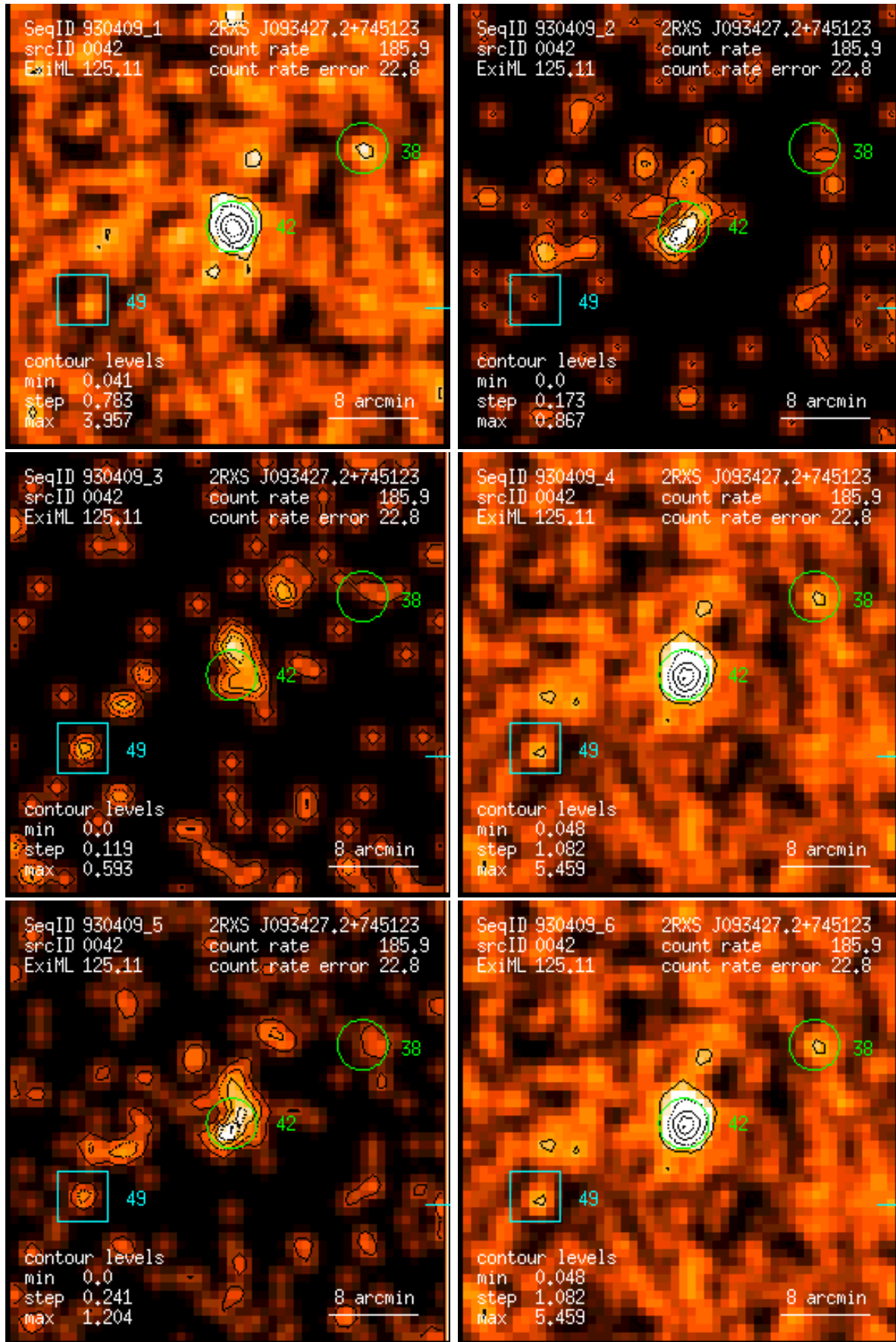
Figure 42: RASS 930409: detection 0042: band rate images, Gaussian filter: (1) PSPC channels 11 – 41, (2) 52 – 90, (3) 91 – 201, (4) 11 – 235, (5) 52 – 201, (6) 11 – 201. Broad band rates in counts/ks. Band rate contour levels in counts/ks/arcmin 2 .
