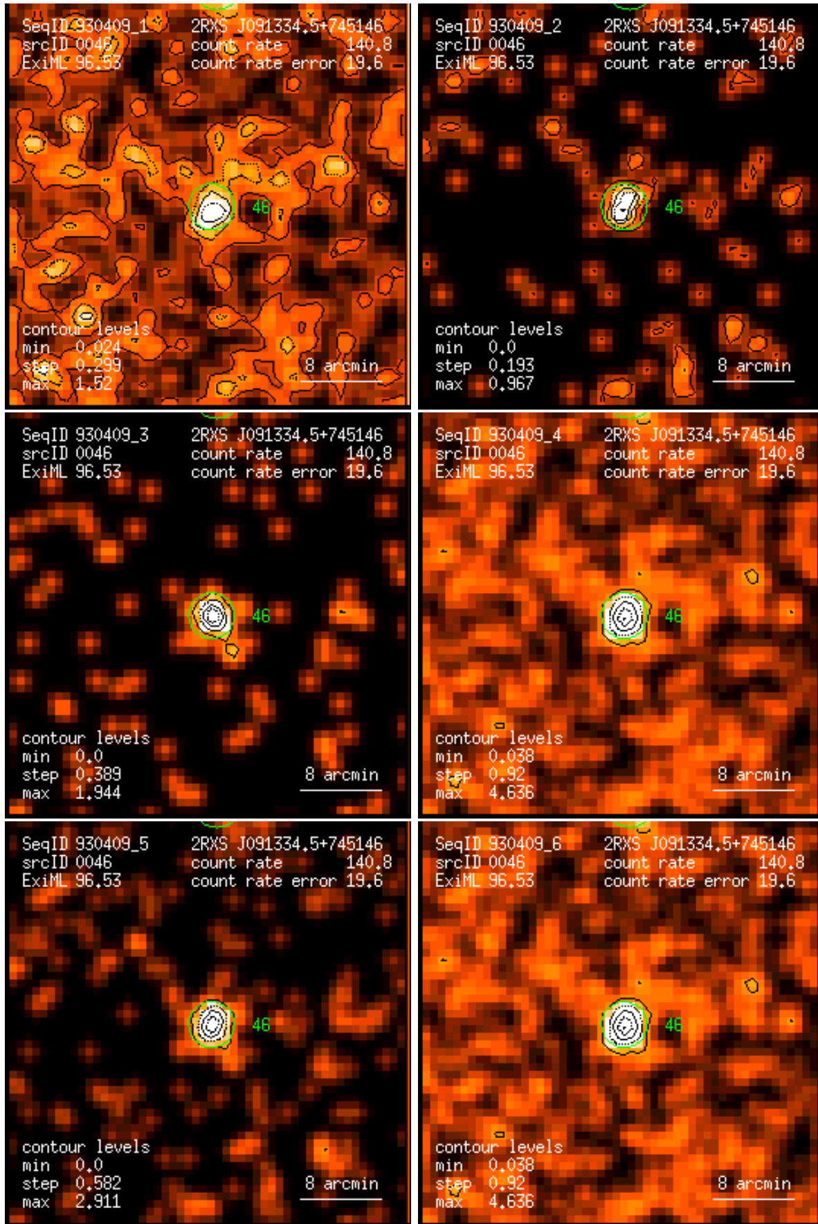
Figure 46: RASS 930409: detection 0046: band rate images, Gaussian filter: (1) PSPC channels 11 – 41, (2) 52 – 90, (3) 91 – 201, (4) 11 – 235, (5) 52 – 201, (6) 11 – 201. Broad band rates in counts/ks. Band rate contour levels in counts/ks/arcmin 2 .
