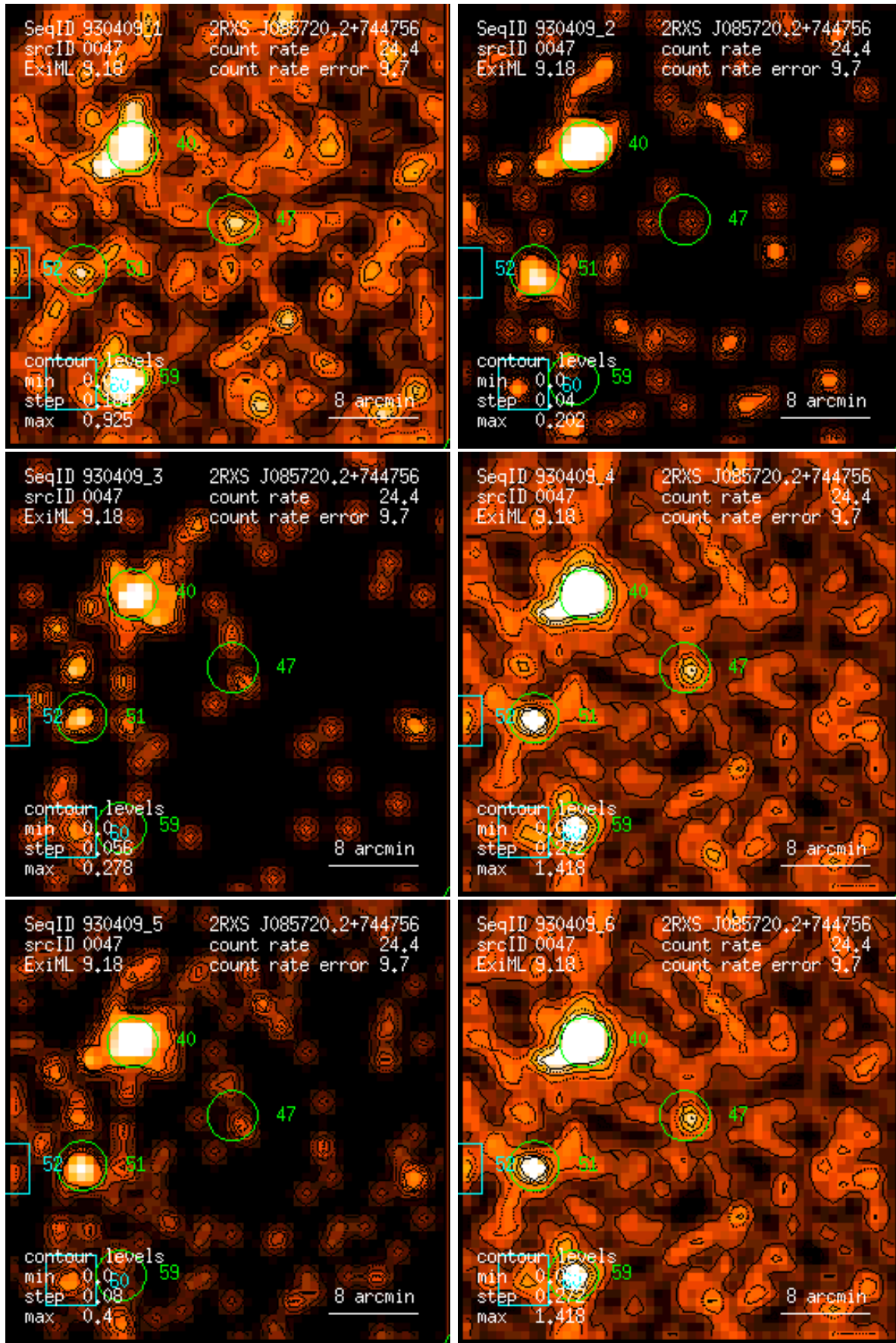
Figure 47: RASS 930409: detection 0047: band rate images, Gaussian filter: (1) PSPC channels 11 – 41, (2) 52 – 90, (3) 91 – 201, (4) 11 – 235, (5) 52 – 201, (6) 11 – 201. Broad band rates in counts/ks. Band rate contour levels in counts/ks/arcmin 2 .
