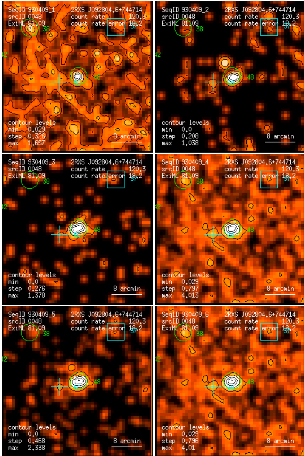
Figure 48: RASS 930409: detection 0048: band rate images, Gaussian filter: (1) PSPC channels 11 – 41, (2) 52 – 90, (3) 91 – 201, (4) 11 – 235, (5) 52 – 201, (6) 11 – 201. Broad band rates in counts/ks. Band rate contour levels in counts/ks/arcmin 2 .
