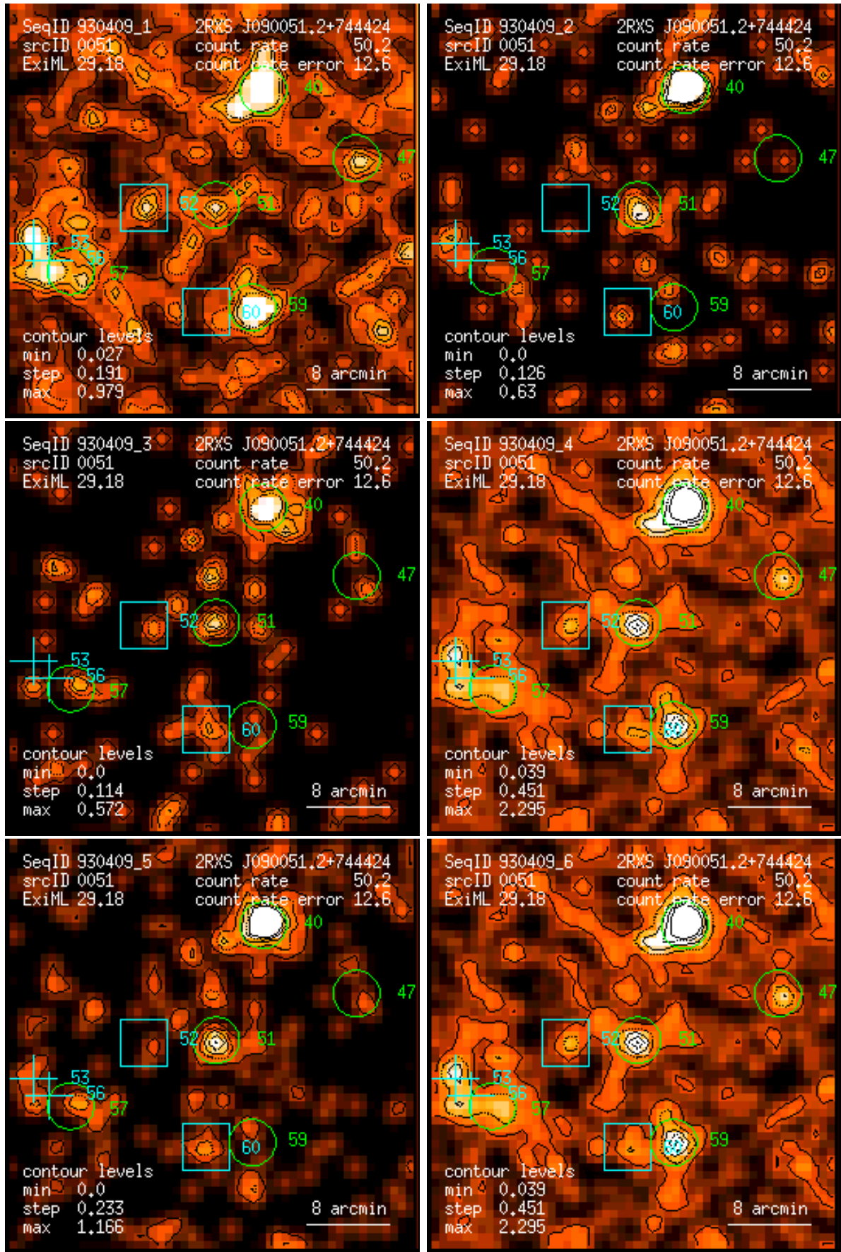
Figure 51: RASS 930409: detection 0051: band rate images, Gaussian filter: (1) PSPC channels 11 – 41, (2) 52 – 90, (3) 91 – 201, (4) 11 – 235, (5) 52 – 201, (6) 11 – 201. Broad band rates in counts/ks. Band rate contour levels in counts/ks/arcmin 2 .
