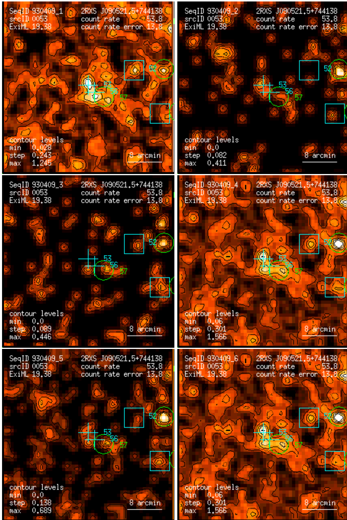
Figure 53: RASS 930409: detection 0053: band rate images, Gaussian filter: (1) PSPC channels 11 – 41, (2) 52 – 90, (3) 91 – 201, (4) 11 – 235, (5) 52 – 201, (6) 11 – 201. Broad band rates in counts/ks. Band rate contour levels in counts/ks/arcmin 2 .
