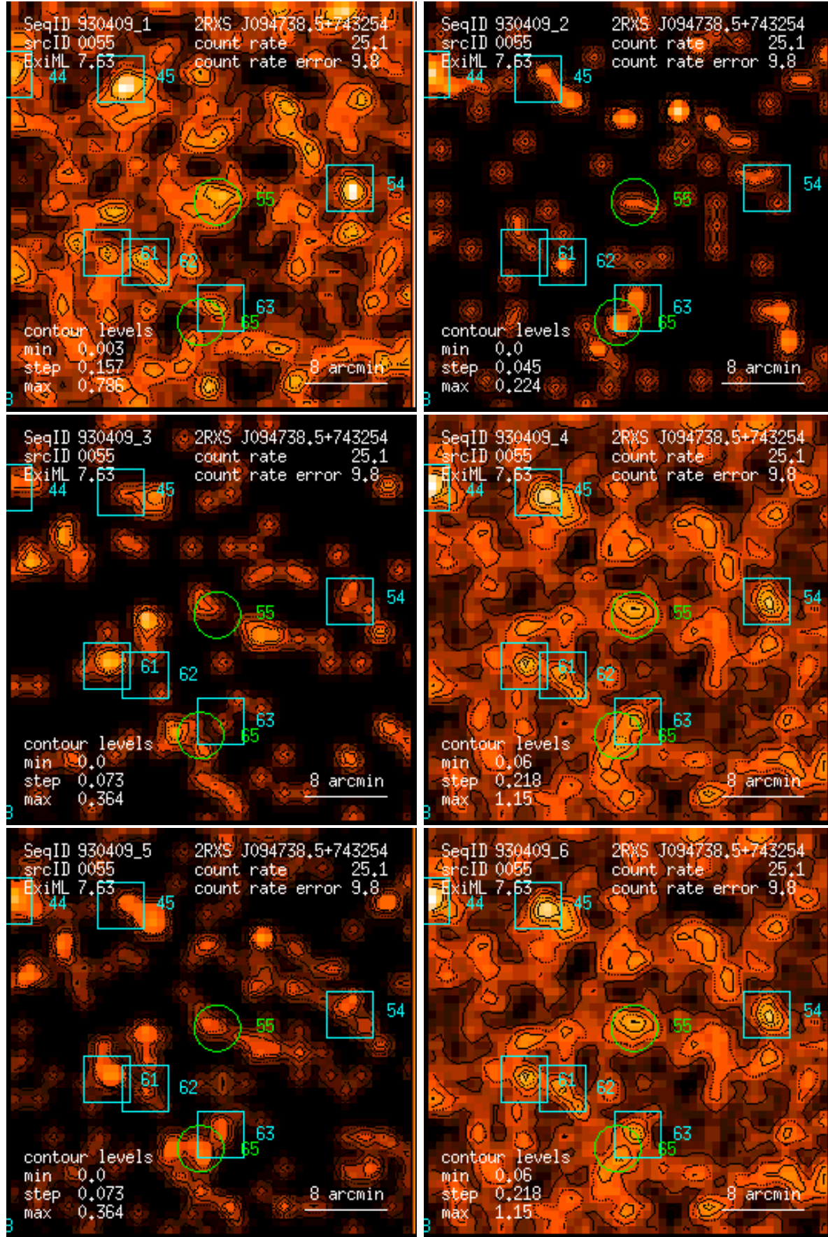
Figure 55: RASS 930409: detection 0055: band rate images, Gaussian filter: (1) PSPC channels 11 – 41, (2) 52 – 90, (3) 91 – 201, (4) 11 – 235, (5) 52 – 201, (6) 11 – 201. Broad band rates in counts/ks. Band rate contour levels in counts/ks/arcmin 2 .
