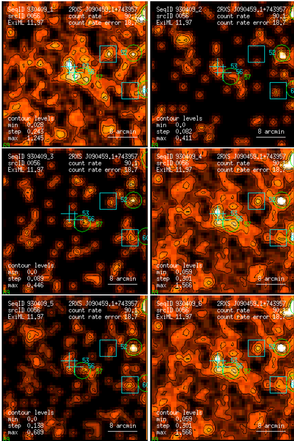
Figure 56: RASS 930409: detection 0056: band rate images, Gaussian filter: (1) PSPC channels 11 – 41, (2) 52 – 90, (3) 91 – 201, (4) 11 – 235, (5) 52 – 201, (6) 11 – 201. Broad band rates in counts/ks. Band rate contour levels in counts/ks/arcmin 2 .
