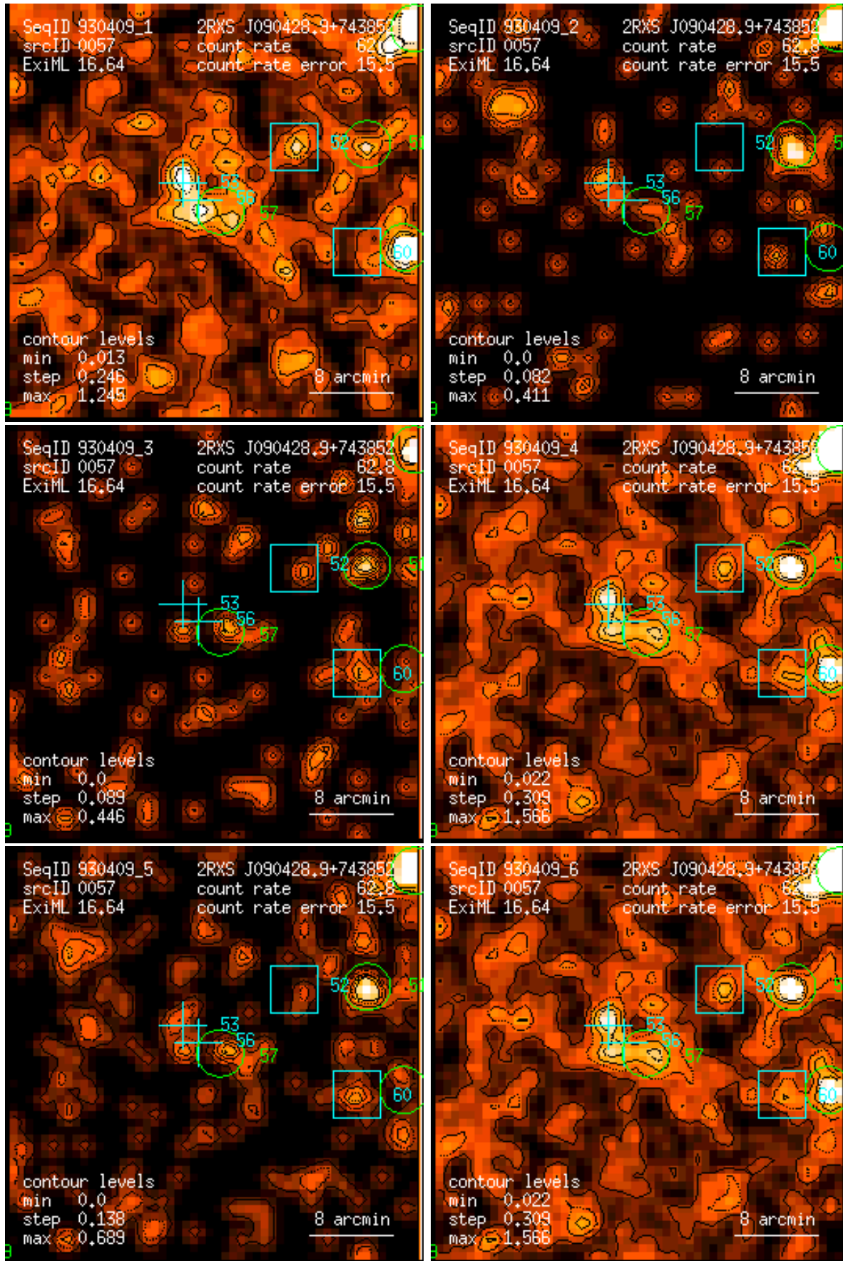
Figure 57: RASS 930409: detection 0057: band rate images, Gaussian filter: (1) PSPC channels 11 – 41, (2) 52 – 90, (3) 91 – 201, (4) 11 – 235, (5) 52 – 201, (6) 11 – 201. Broad band rates in counts/ks. Band rate contour levels in counts/ks/arcmin 2 .
