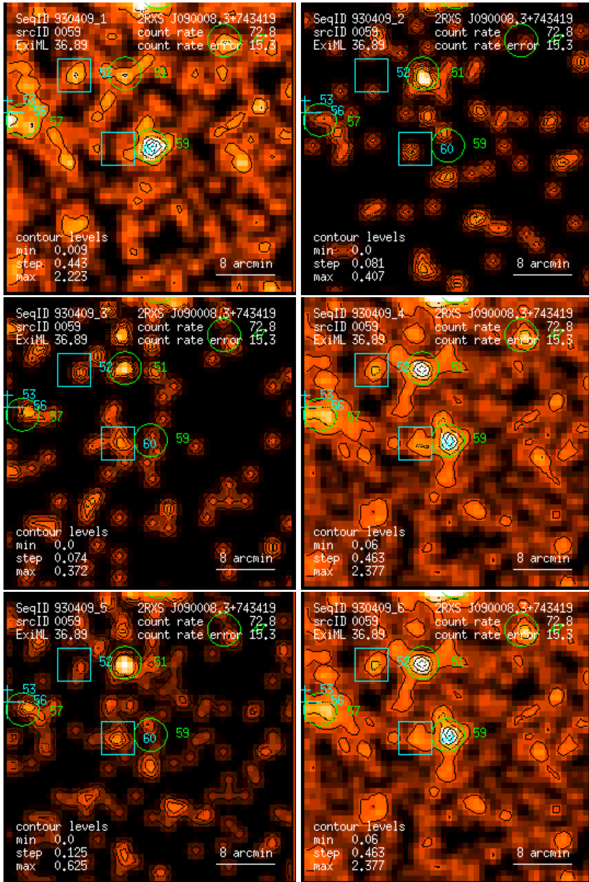
Figure 59: RASS 930409: detection 0059: band rate images, Gaussian filter: (1) PSPC channels 11 – 41, (2) 52 – 90, (3) 91 – 201, (4) 11 – 235, (5) 52 – 201, (6) 11 – 201. Broad band rates in counts/ks. Band rate contour levels in counts/ks/arcmin 2 .
