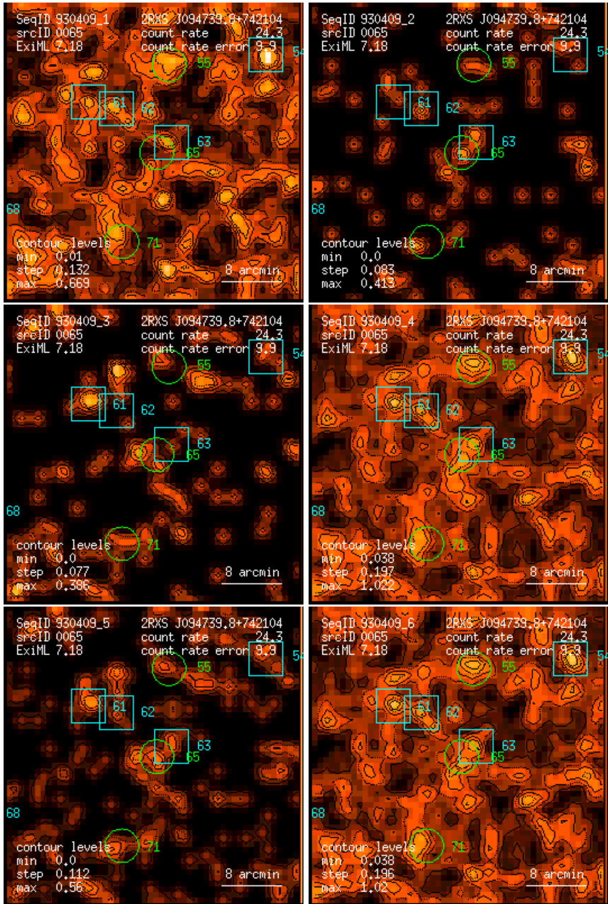
Figure 65: RASS 930409: detection 0065: band rate images, Gaussian filter: (1) PSPC channels 11 – 41, (2) 52 – 90, (3) 91 – 201, (4) 11 – 235, (5) 52 – 201, (6) 11 – 201. Broad band rates in counts/ks. Band rate contour levels in counts/ks/arcmin 2 .
