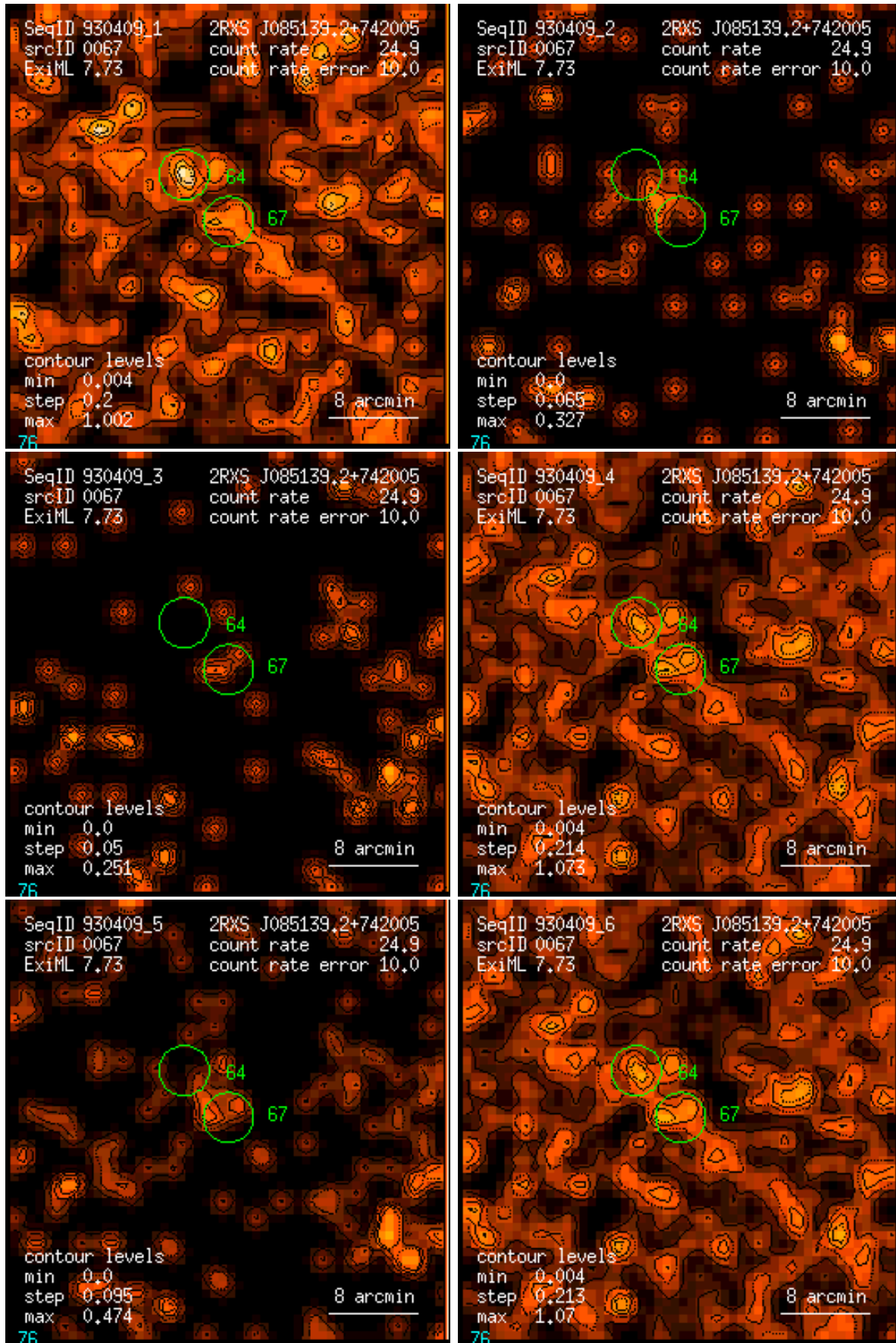
Figure 67: RASS 930409: detection 0067: band rate images, Gaussian filter: (1) PSPC channels 11 – 41, (2) 52 – 90, (3) 91 – 201, (4) 11 – 235, (5) 52 – 201, (6) 11 – 201. Broad band rates in counts/ks. Band rate contour levels in counts/ks/arcmin 2 .
