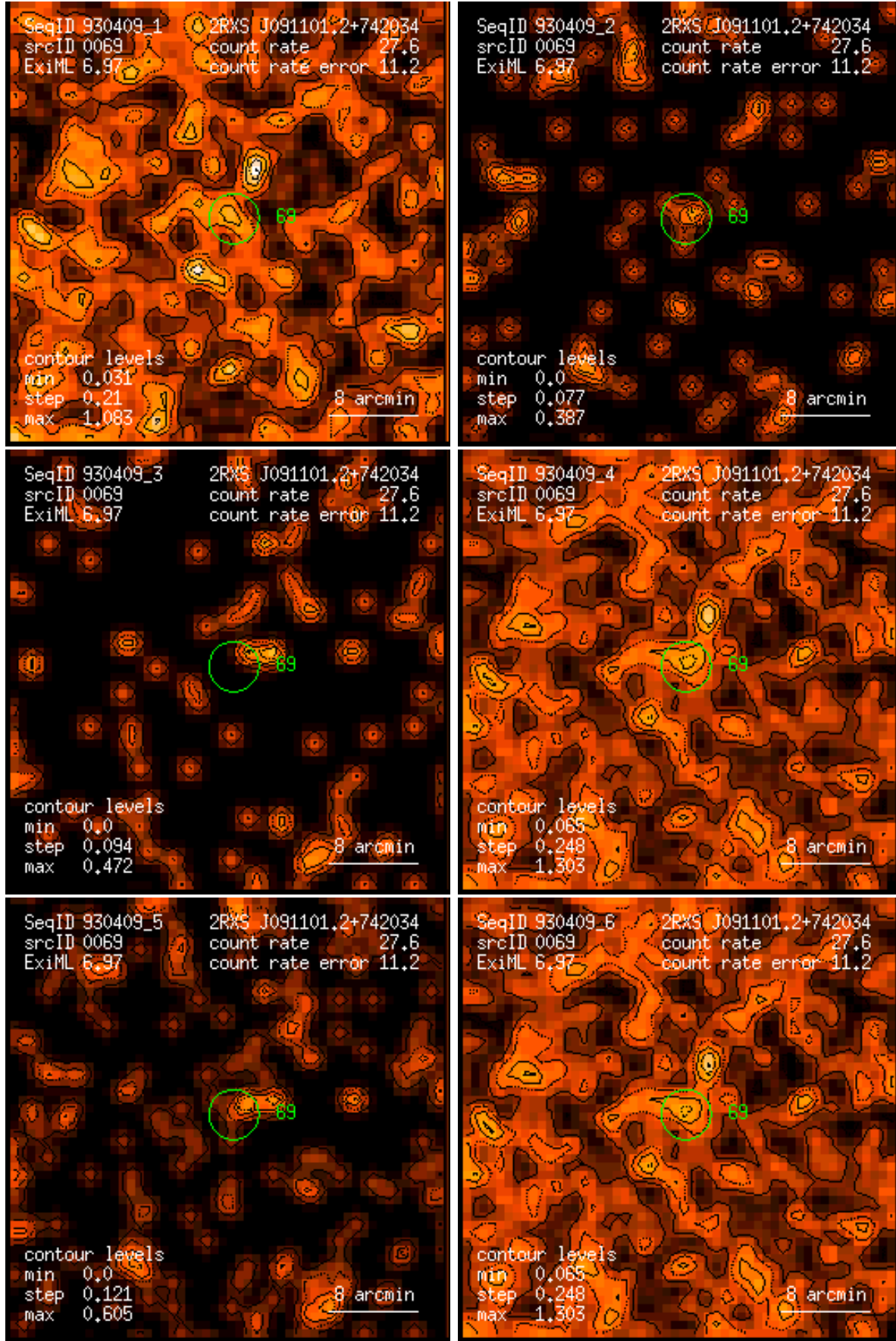
Figure 69: RASS 930409: detection 0069: band rate images, Gaussian filter: (1) PSPC channels 11 – 41, (2) 52 – 90, (3) 91 – 201, (4) 11 – 235, (5) 52 – 201, (6) 11 – 201. Broad band rates in counts/ks. Band rate contour levels in counts/ks/arcmin 2 .
