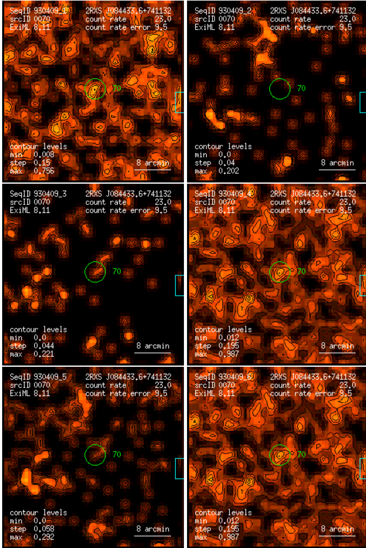
Figure 70: RASS 930409: detection 0070: band rate images, Gaussian filter: (1) PSPC channels 11 – 41, (2) 52 – 90, (3) 91 – 201, (4) 11 – 235, (5) 52 – 201, (6) 11 – 201. Broad band rates in counts/ks. Band rate contour levels in counts/ks/arcmin 2 .
